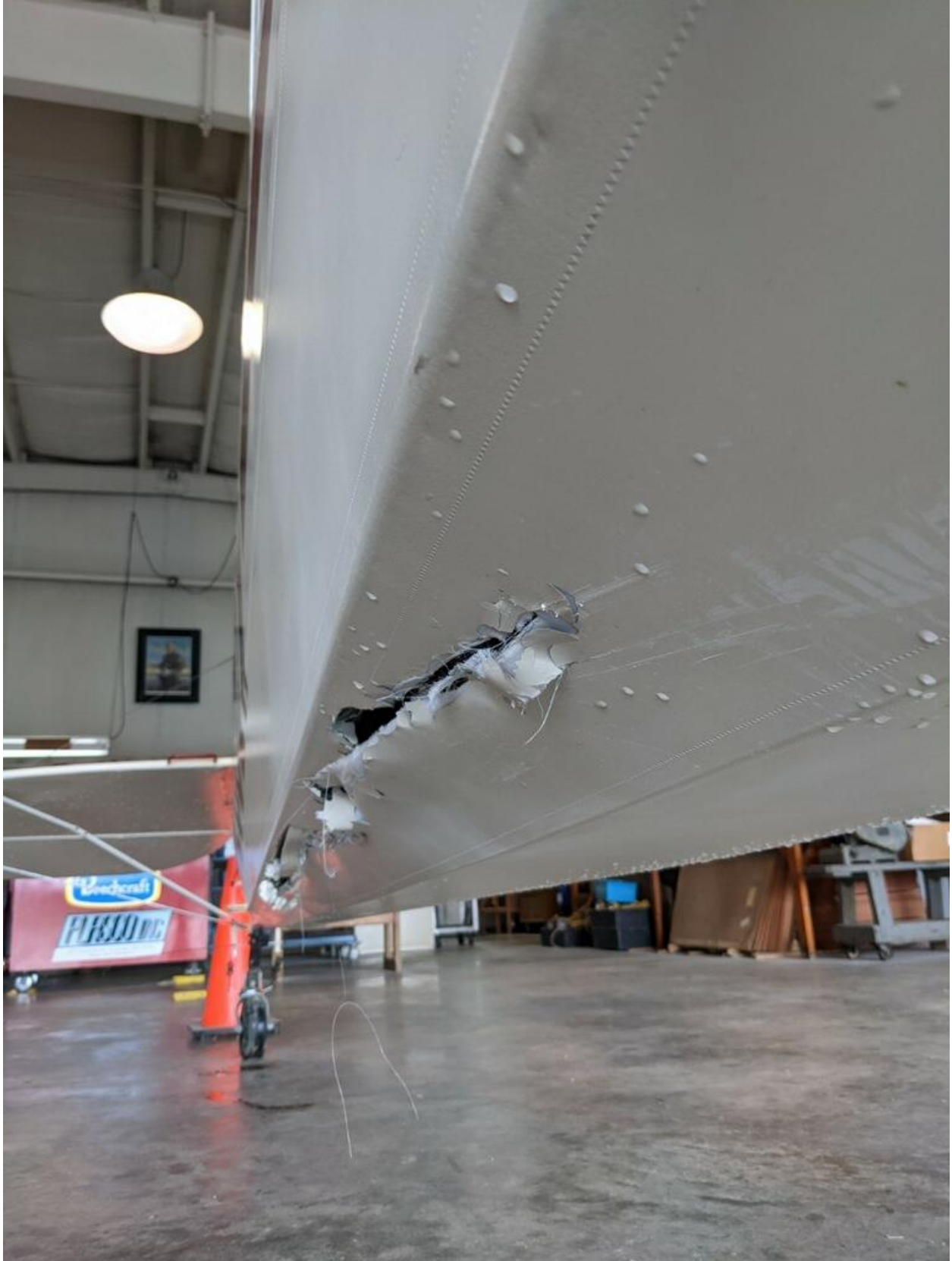
Photo 1: Fuselage Damage (Source – FAA)
