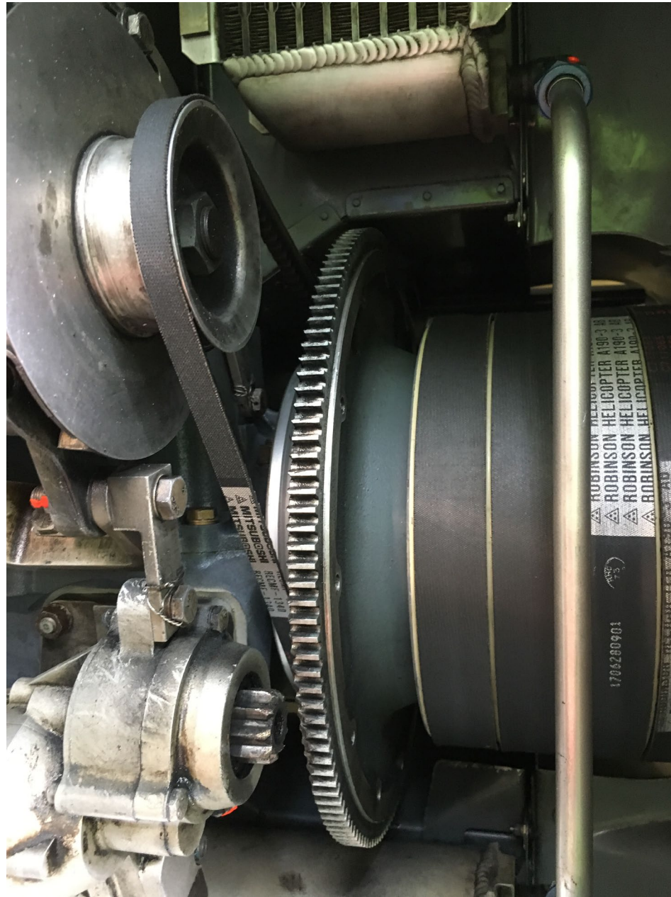
Photo 2 – Damage to the Starter Ring and Starter Teeth
