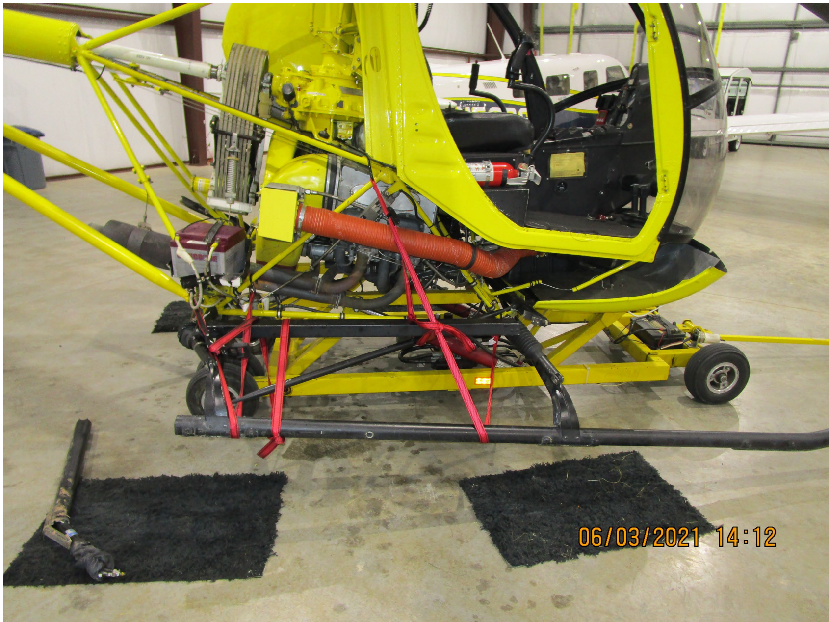
Photo 2 – Damage to fuselage structure
