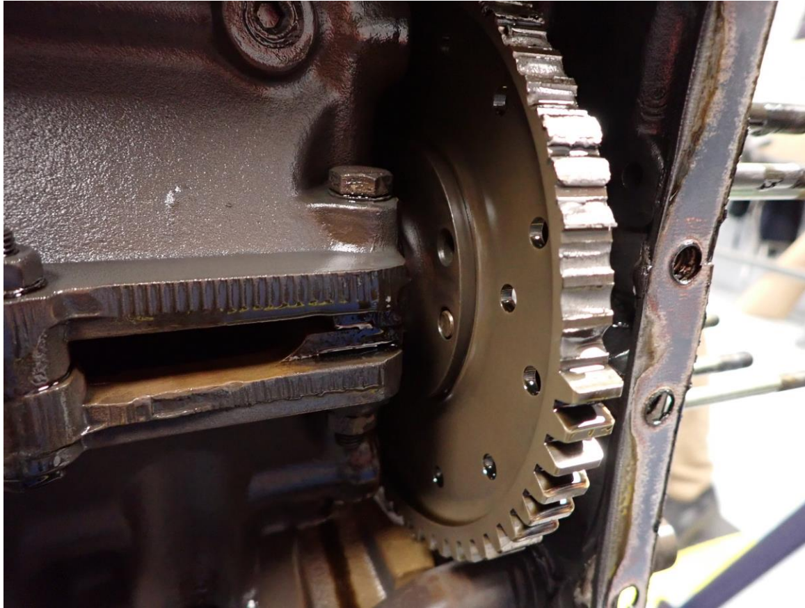
Photograph 3 - Missing Teeth on Camshaft Gear
