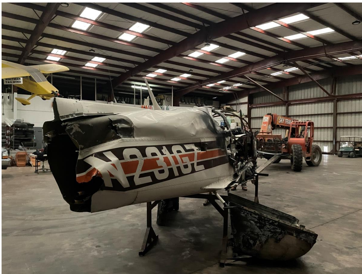
Photograph 1 - Substantially Damaged Airplane (Courtesy of FAA)
