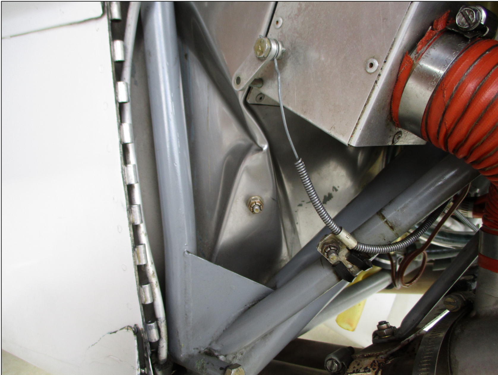
Photo 2 – View of the damaged firewall (Photo Courtesy of FAA)
