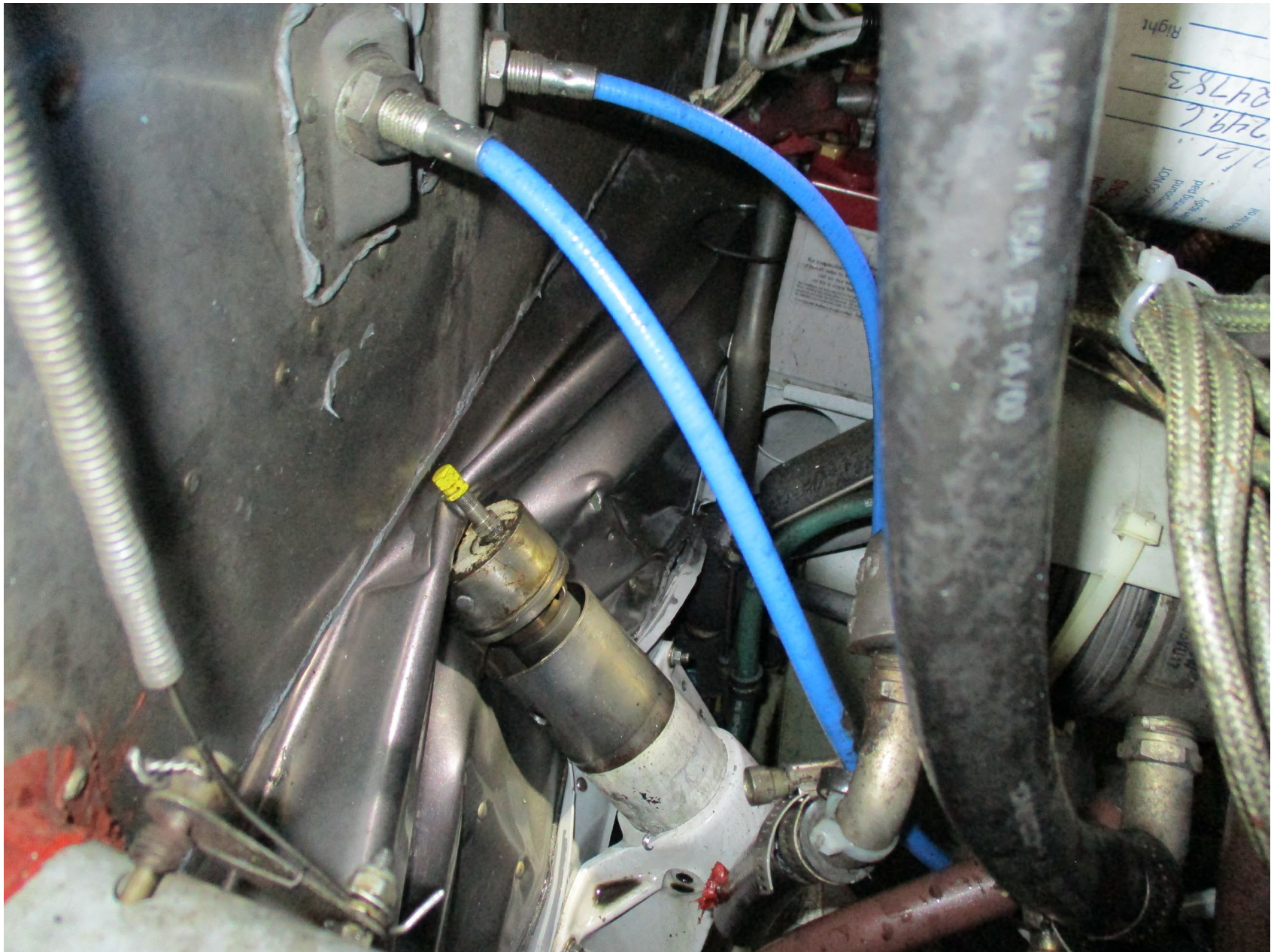
Photo 1 – View of Engine Firewall (photo provided by FAA)
