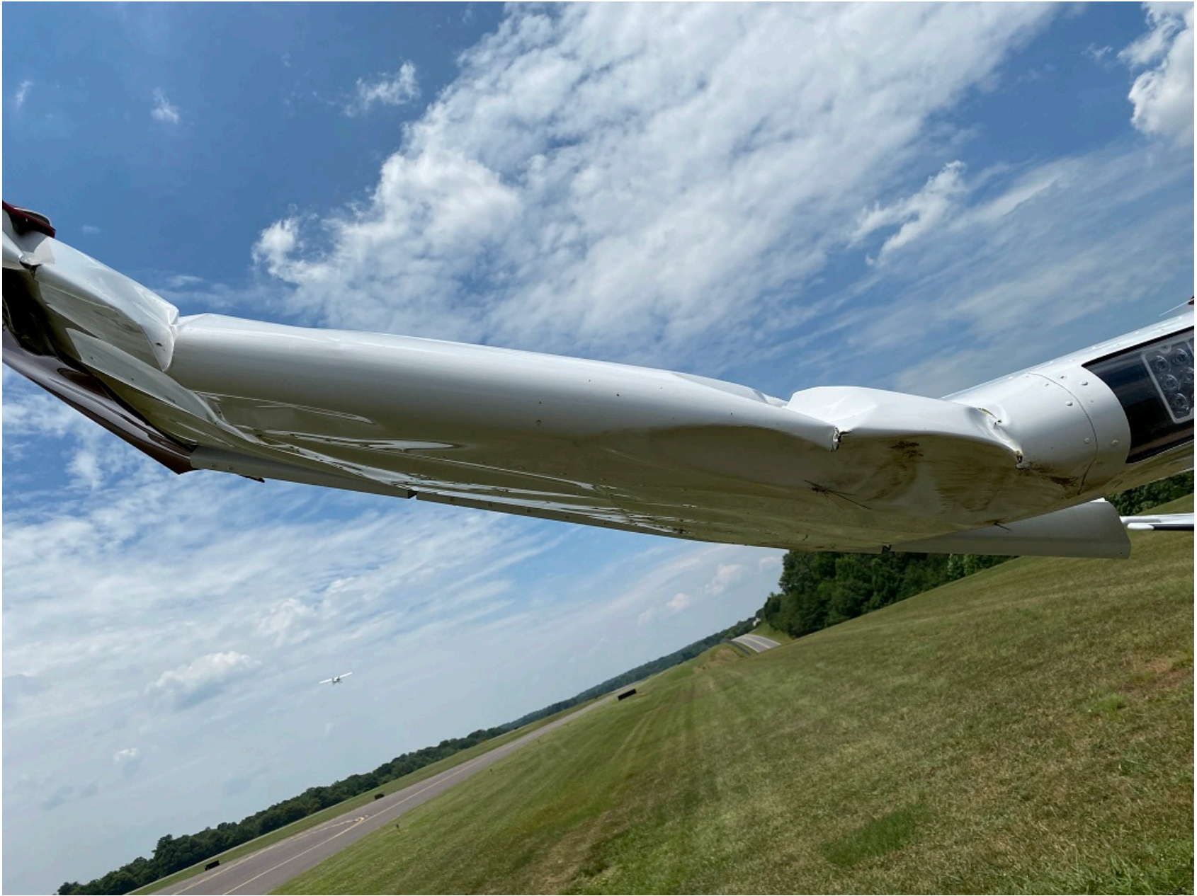
Photo 3 – Right Wing Damage (Photo Courtesy of FAA)
