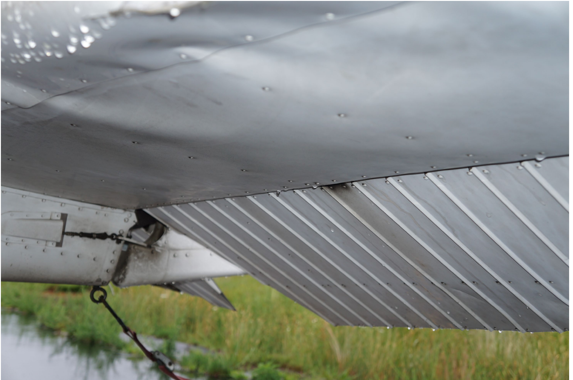
Photo 2 - Horizontal Stabilizer Damage (FAA Photo)
