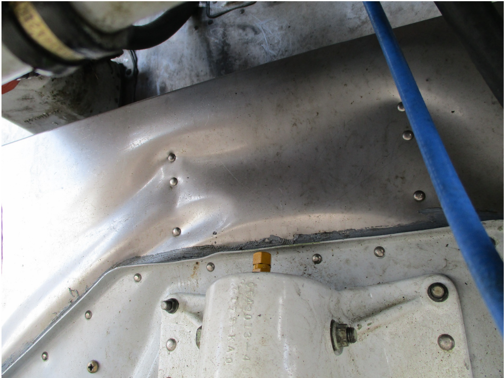
Photo 3 – View of Firewall Damage (Photo Courtesy of Box Aviation)
