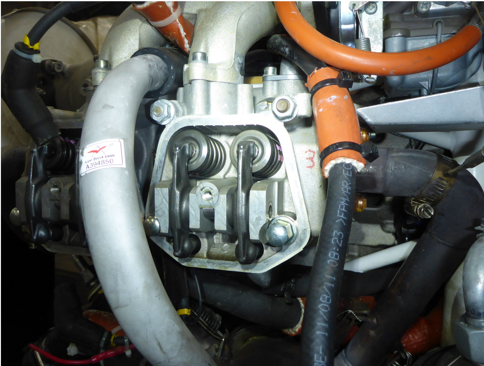
Photo 4: View of the number 3 cylinder head. (Photo Courtesy of Rotax)
