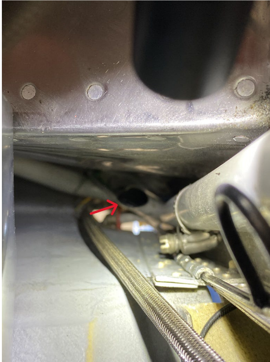
Photograph 4 - Second Separated Frame Tube (Courtesy of FAA)
