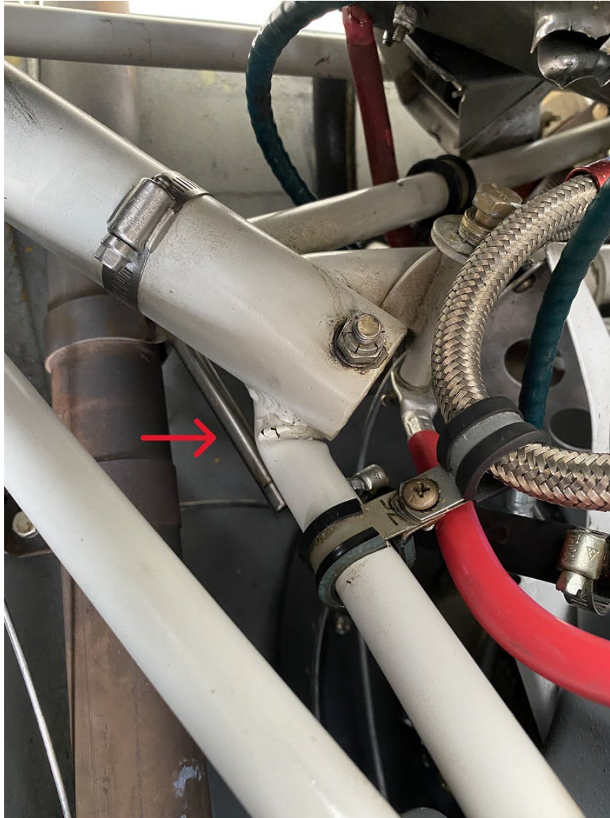
Photograph 2 - Bent Frame Tube (Courtesy of FAA)
