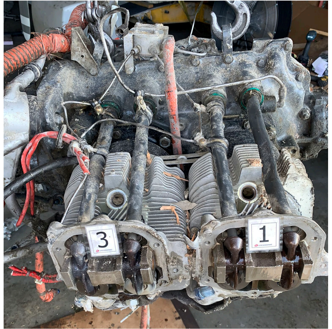
Photo 10: View of engine after removal of valve covers at exam location. (Courtesy of Lycoming)
