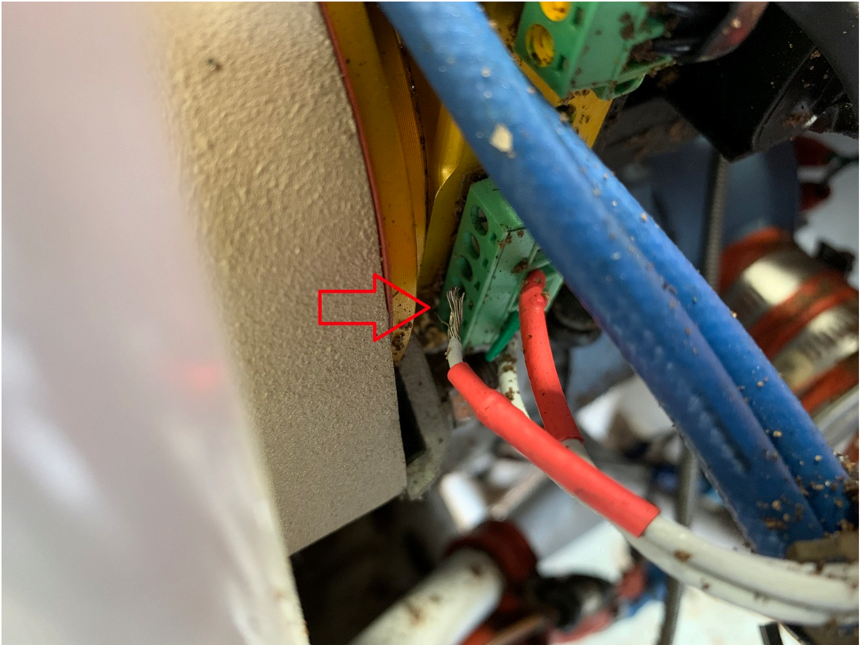
Photo 3 – Loose wire (Magneto)
