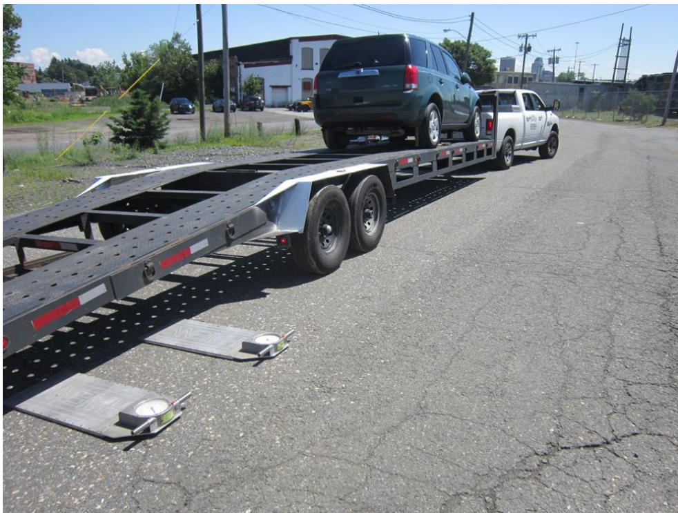
Photo 12. Massachusetts State Police Weighing Westfield Transport Vehicle
