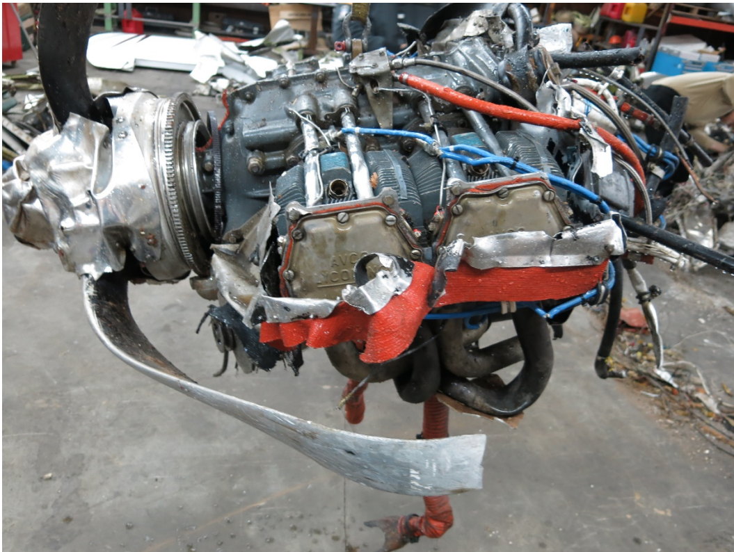
Photograph 5 – Engine, left side.
