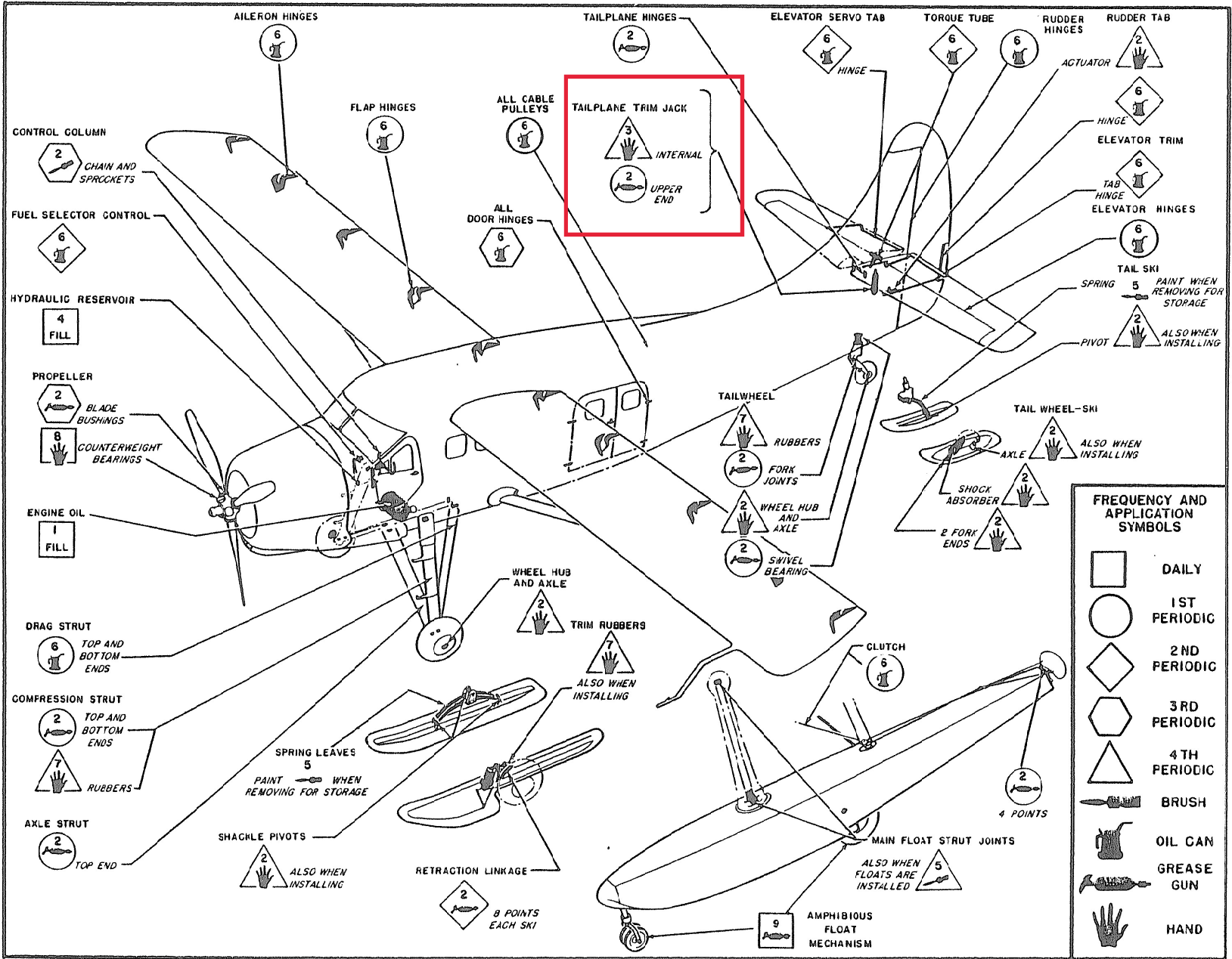
Figure 1-14 Lubrication Diagram
