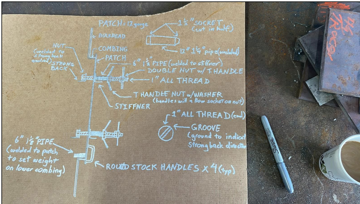
Figure 2 - Early planning for replacement hatches
