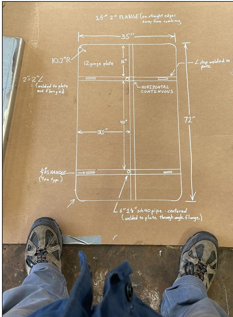
Figure 3 - Hatch drawings
