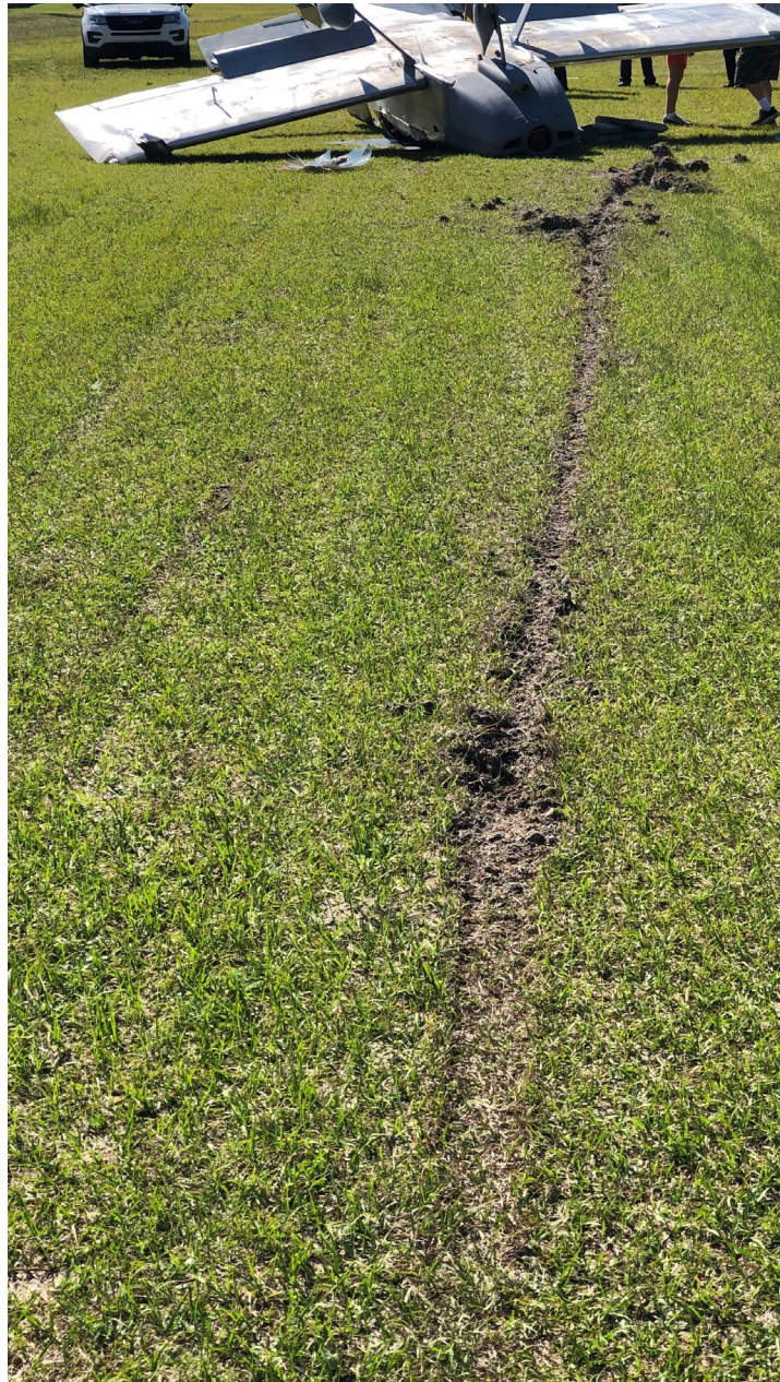
Photo 1 – Digital Photograph Provided by FAA. View Depicting the Ground Scar on the Runway Made by the Nose Landing Gear and the Inverted Airplane.
