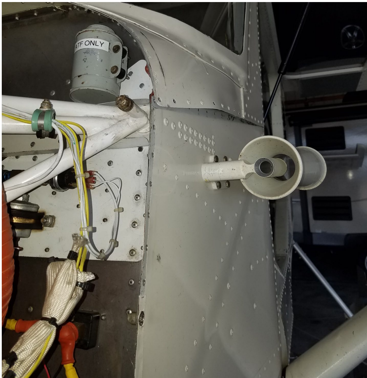
Photograph 2 2 – Accident airplane, fuselage damage.
