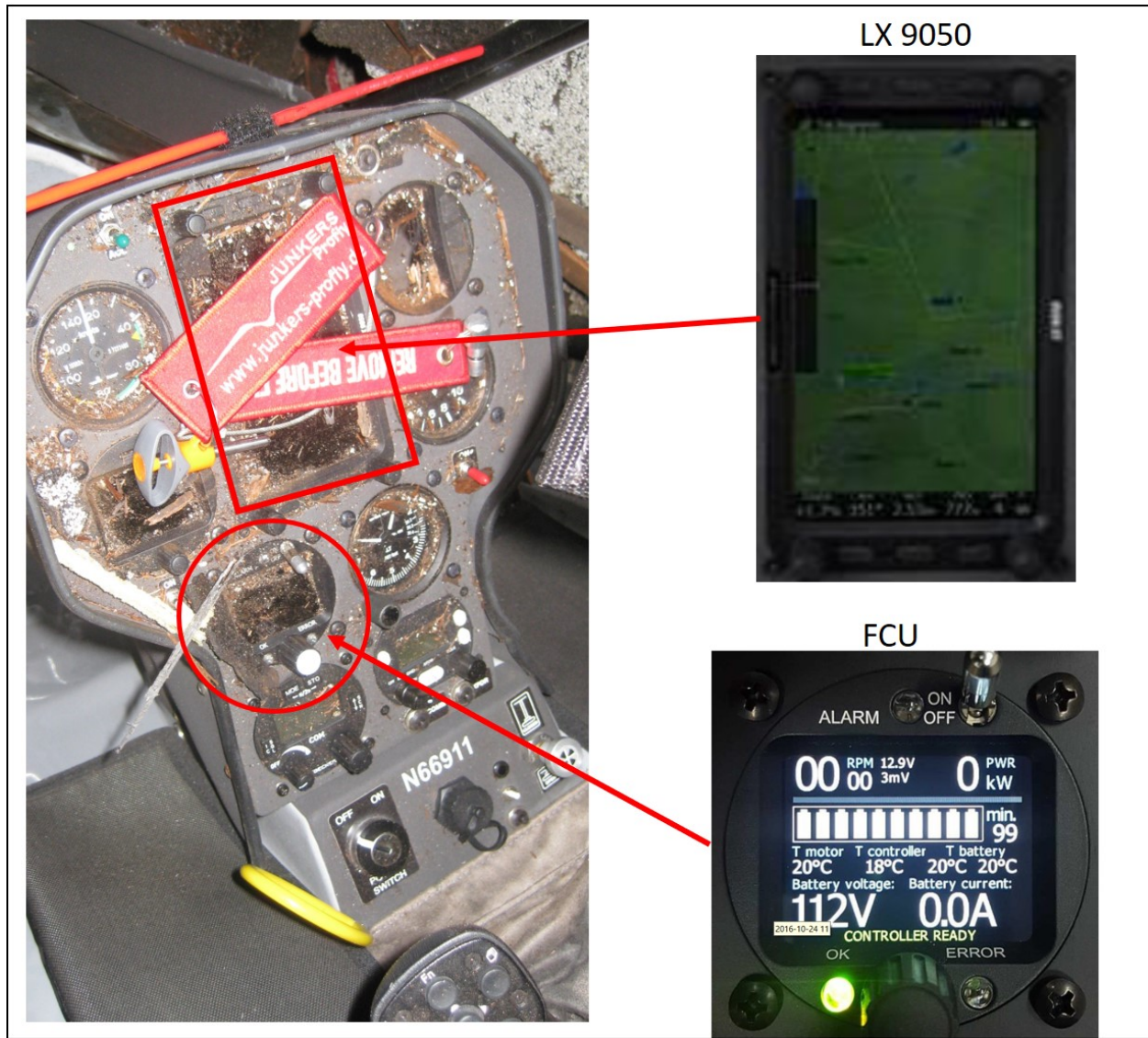
Photograph 4 4 – Instrument panel.
