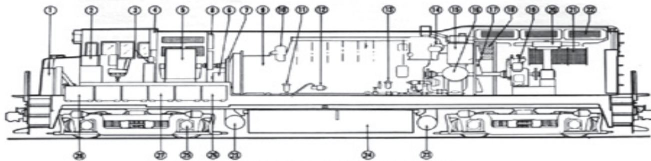
Fig. 22-B U MODEL LOCOMOTIVE
