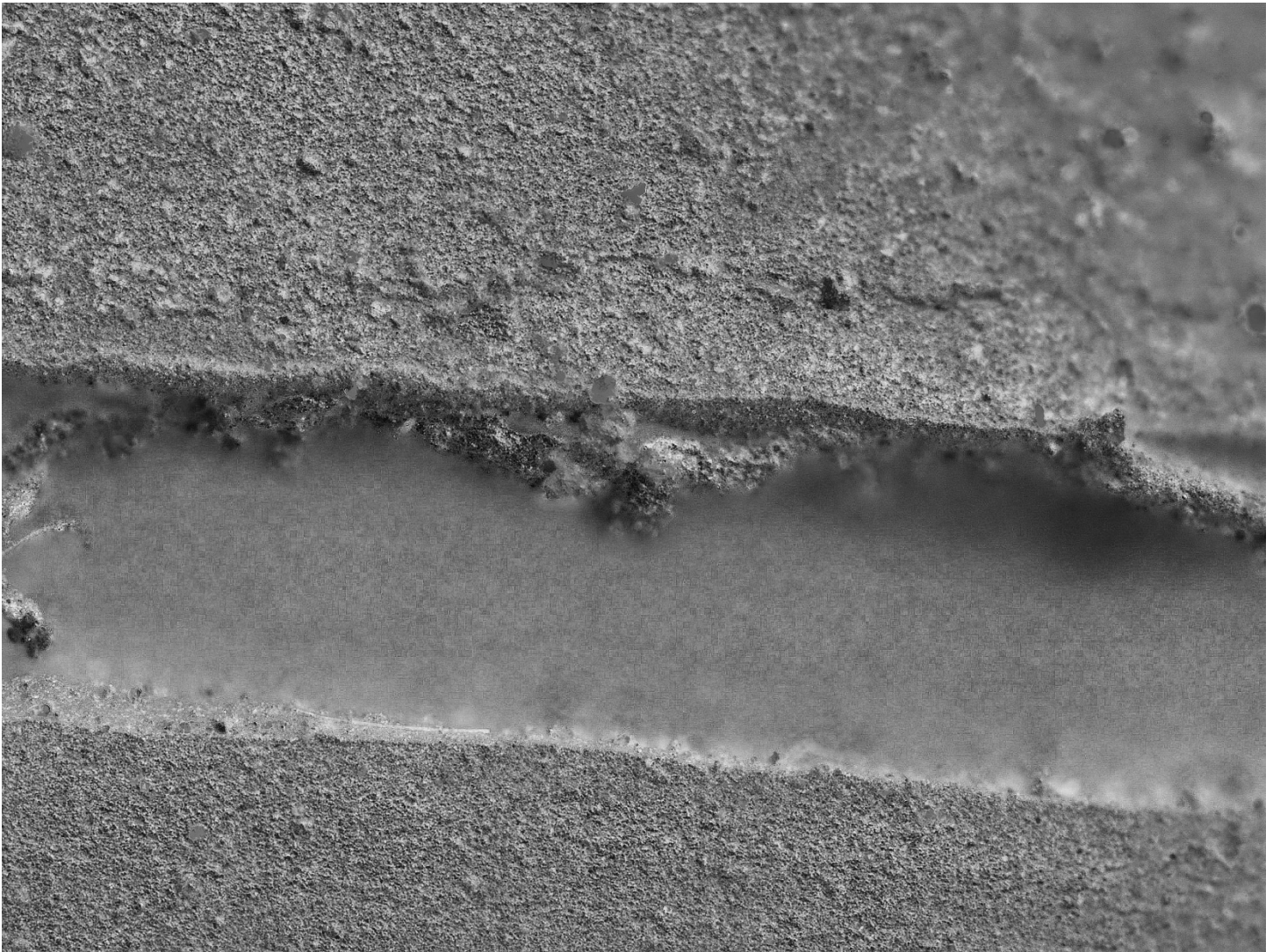
Figure 5. Micrograph of surface split in exemplar gasket (HMD22LR001-HAZ-005 taken from TILX731779 (line 37))
