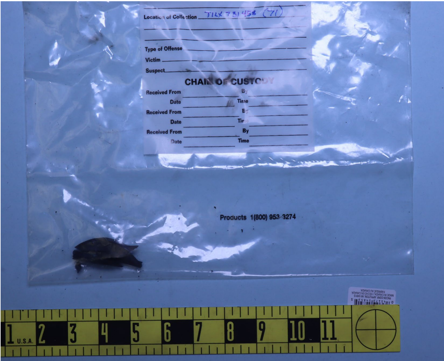
Figure 3. Damaged portion of gasket (HMD22LR001-HAZ-006 taken from TILX731458 (line 71))
