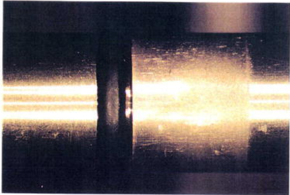
Figure 6.3 Accident Pilot Valve Poppet Shaft
