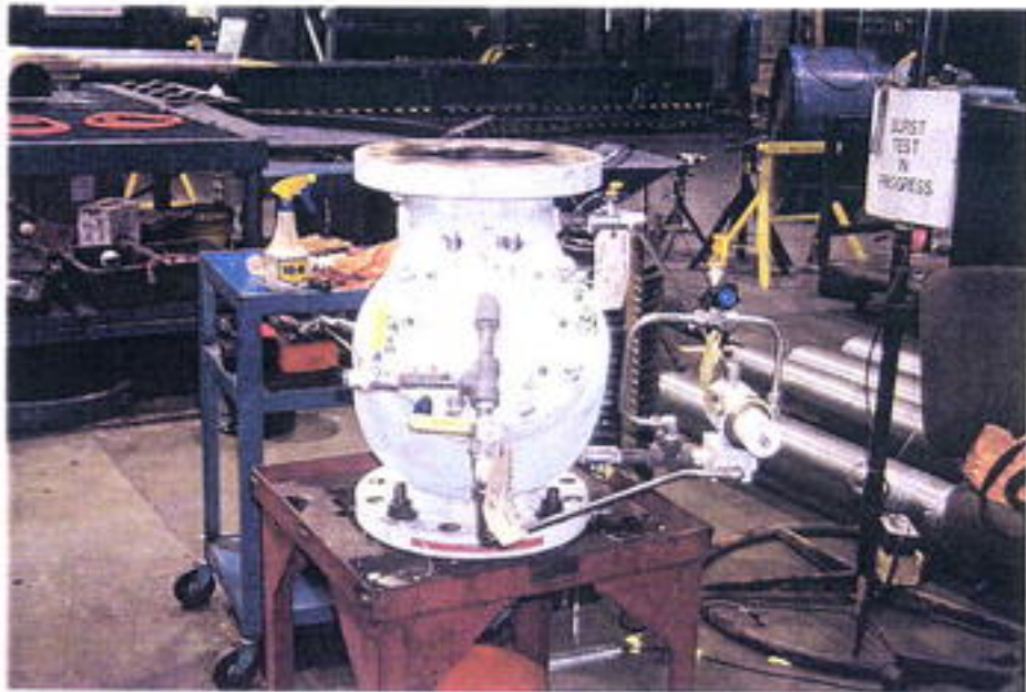
Figure 6.15 Reassembled Relief Valve
