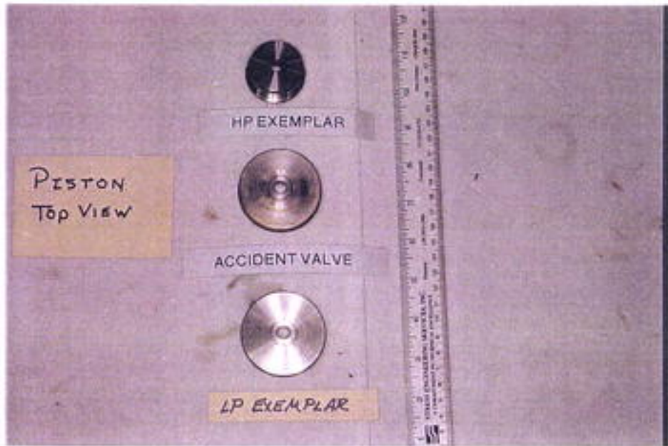
Figure 5.8 Pistons from Pilot Valves
