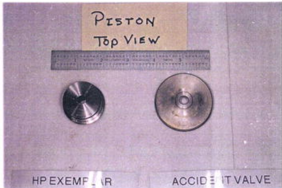
Figure 5.3 Pistons from HP Exemplar and Accident Pilot Valves
