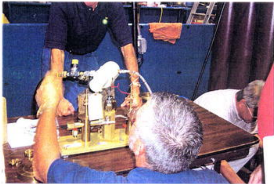
Figure 4.2 Dead Weight Test Set-up
