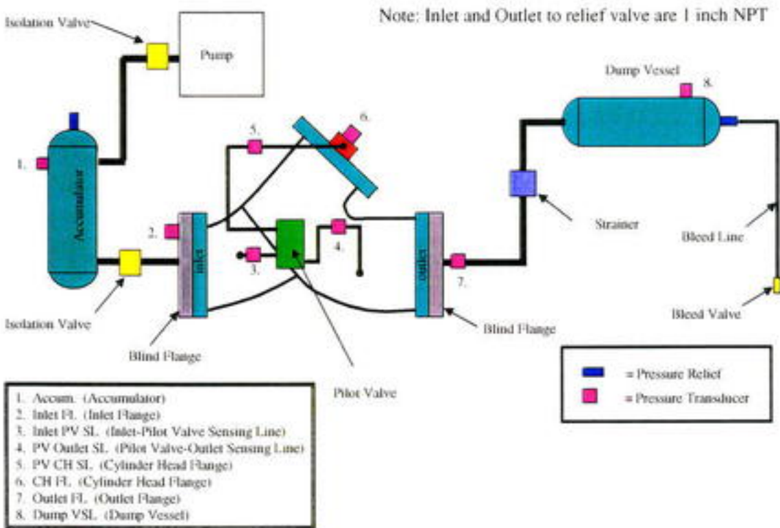
Figure 3.1 Test Set-up for As-received Valve
