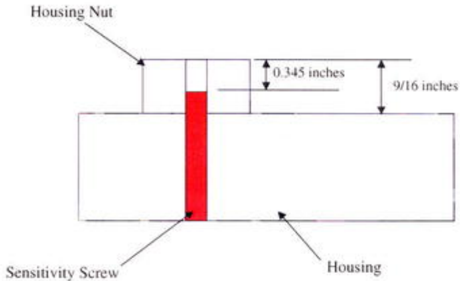
Figure 2.14 Measurements of Sensitivity Screw Location
