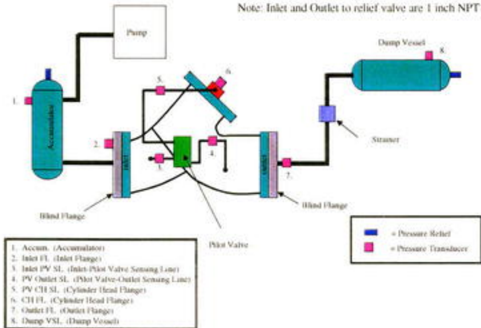
Figure 2.13 Revised Test Set-up
