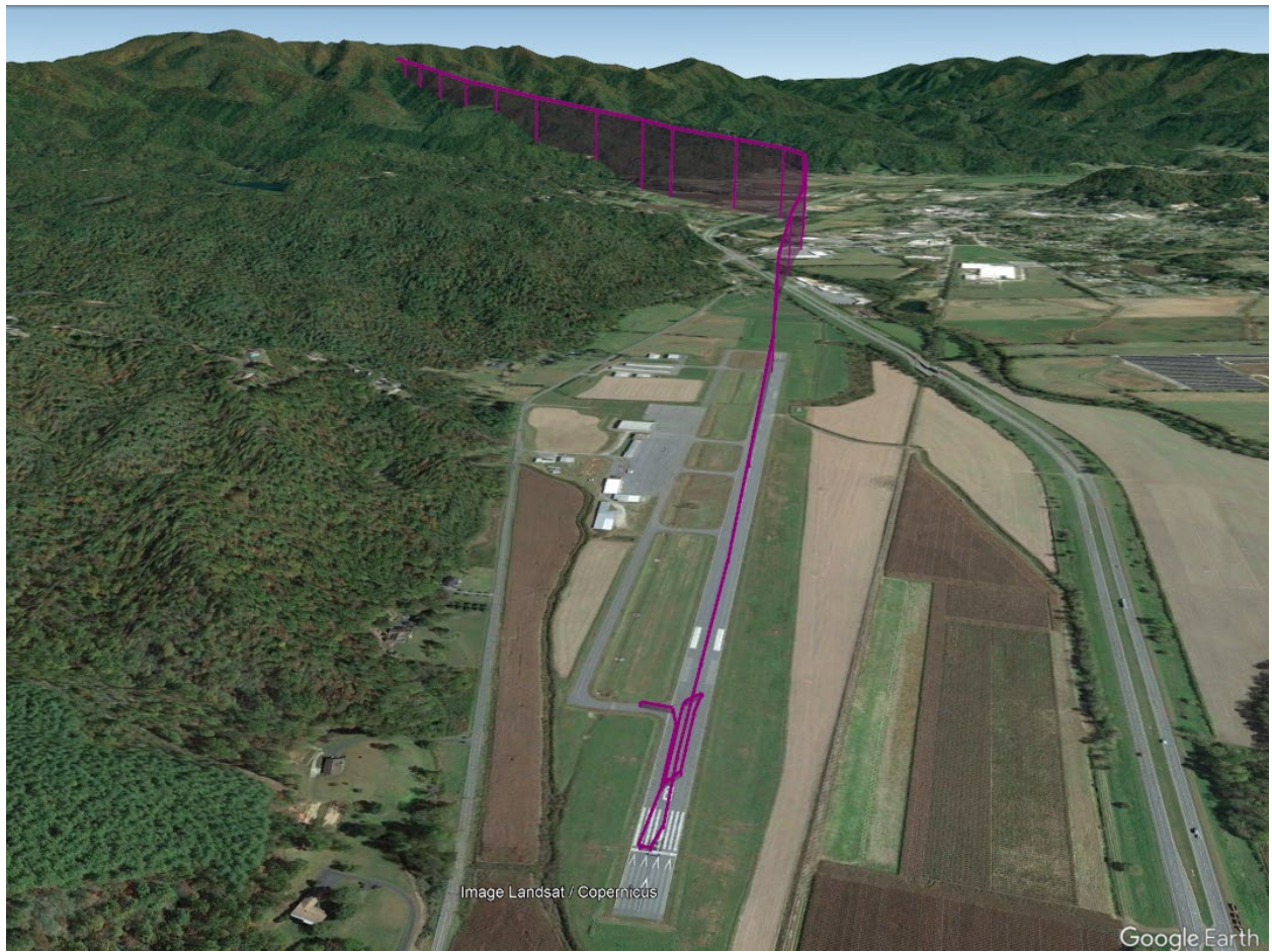
Airplane's GPS-derived departure track (magenta overlay) from runway 8 toward the rising terrain northeast of the airport.
