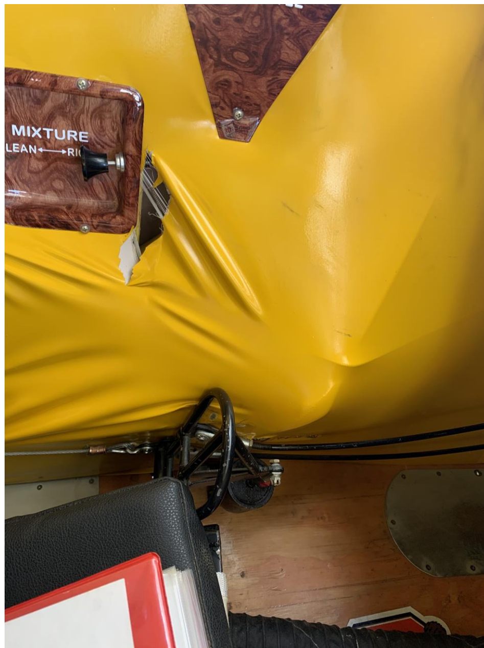
Photo 4 – Accident airplane left cabin fuselage. (Courtesy of the FAA)
