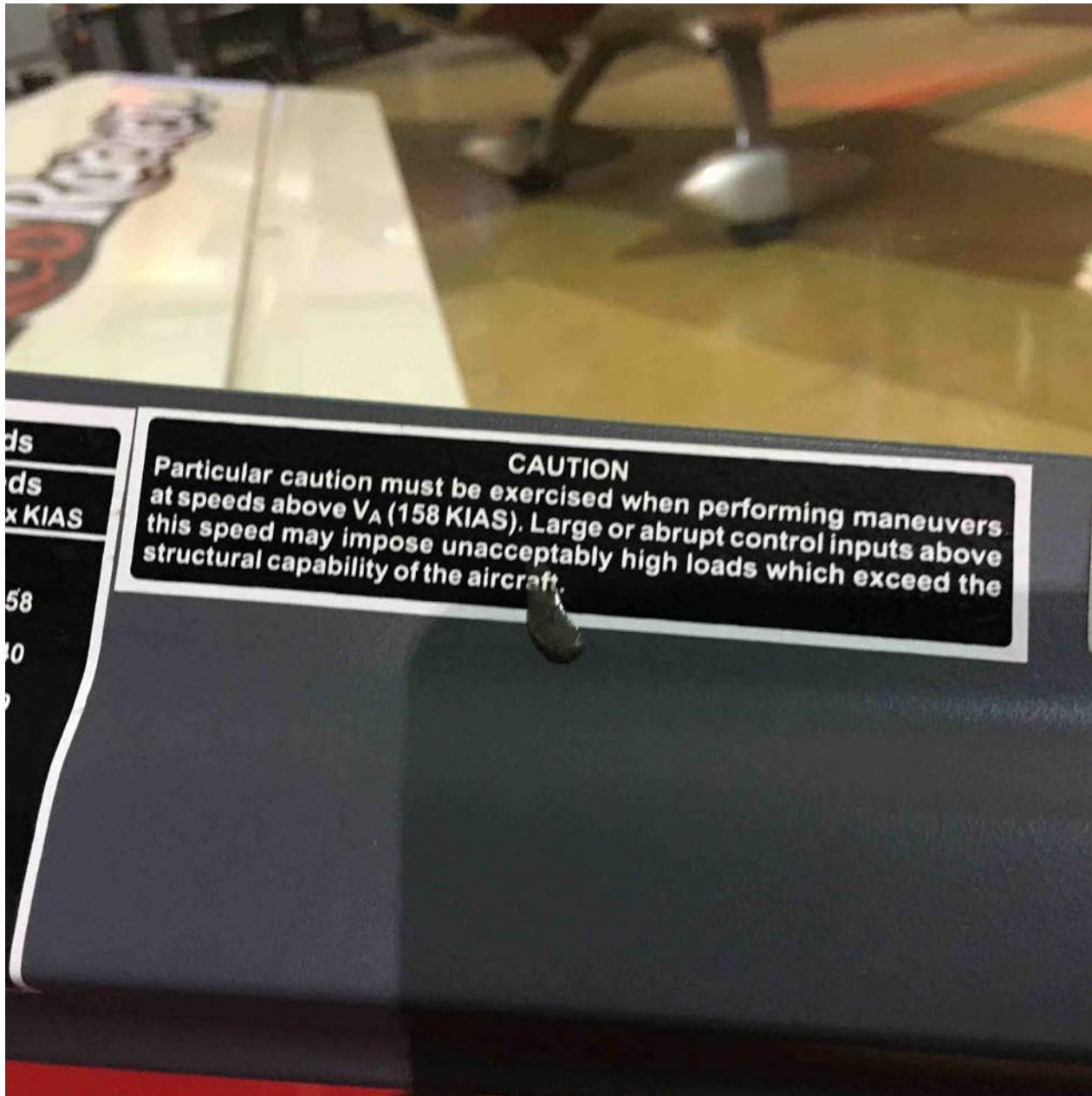
Photo 2 – Maneuvering Speed Placard
