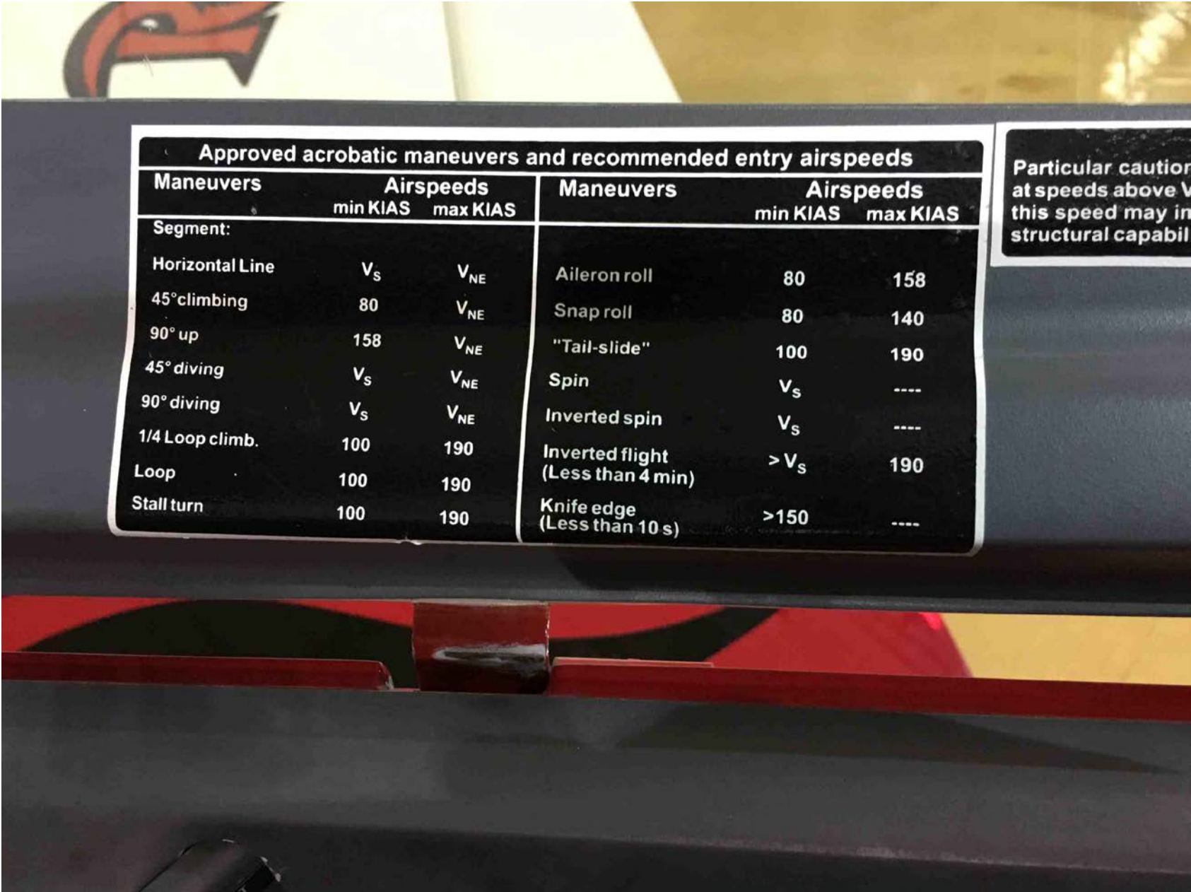
Photo 1 – Speeds Placard
