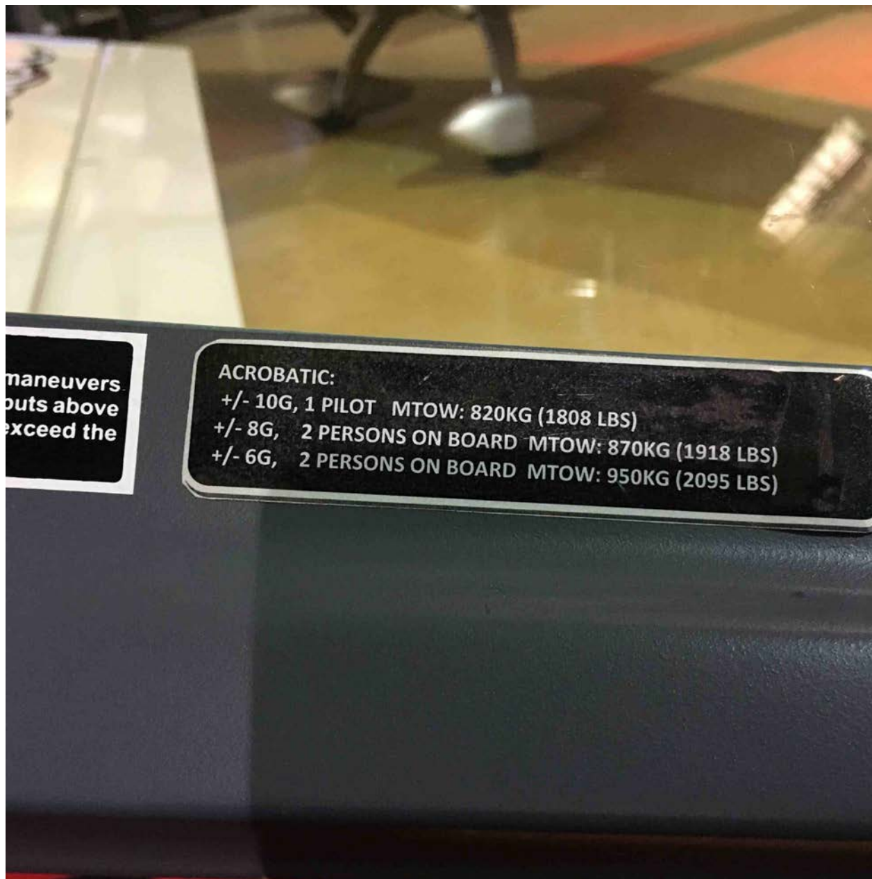
Photo 3 – G Limit Placard Acrobatic Category
