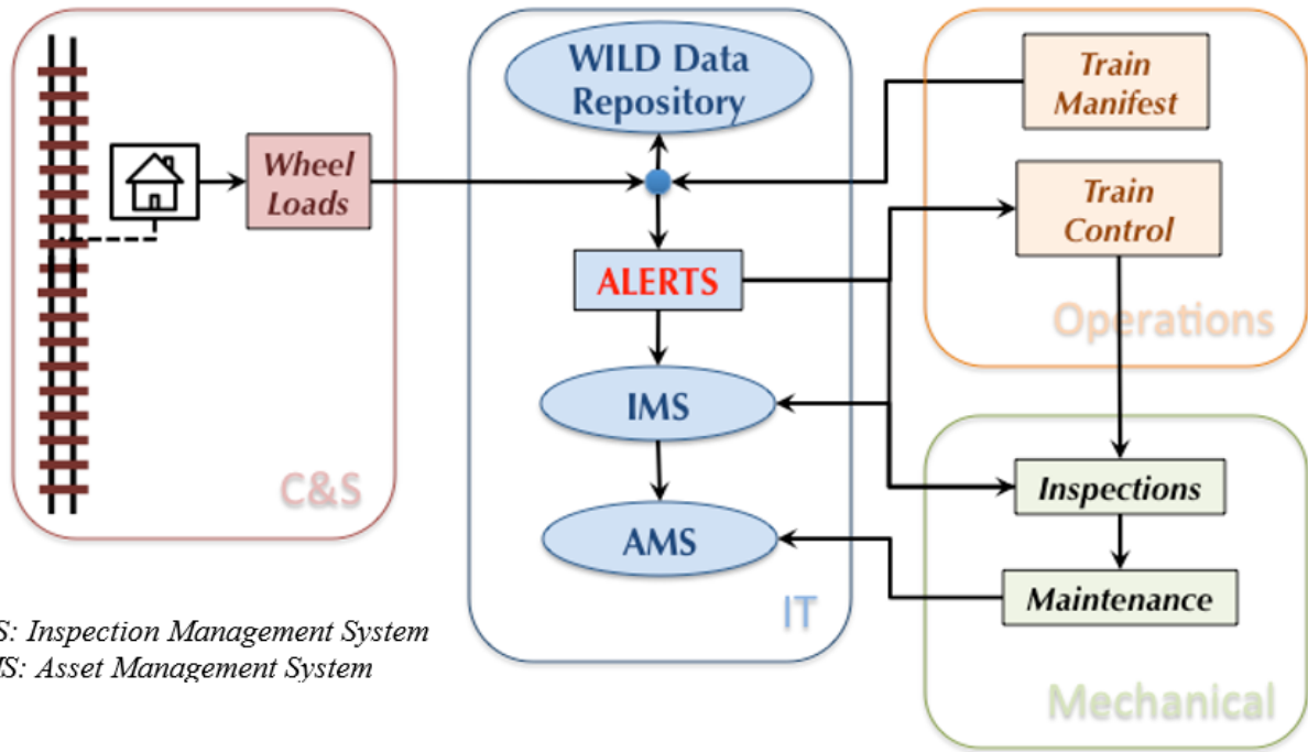
Figure 4-12. Interdepartmental data flow for MNR's WILD system [1]
