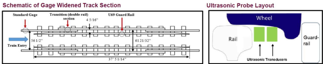
Figure 3-5. Schematic plan of track structure (wide gauge, guard-rail) for ACWD site [30]
