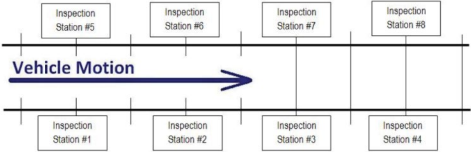
Figure 3-7. Schematic plan of ACWD site developed by Nordco [26]
