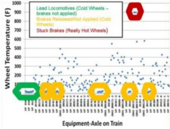
Figure 3-25. An example of WTD for brake effective tests (left); (right) Wheel temperature variation on a train indicating braking condition [8]
