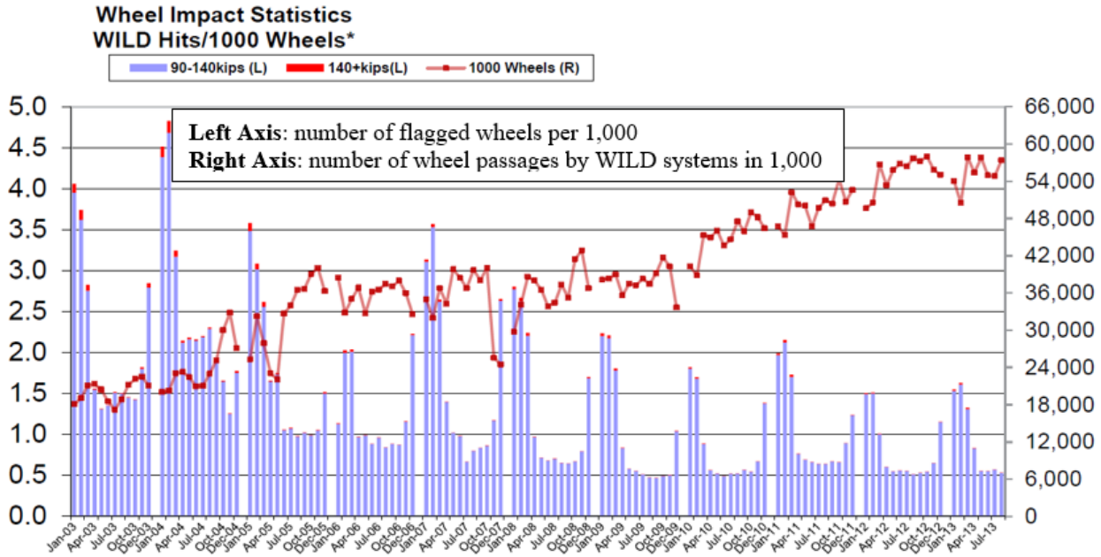
Figure 4-10. Rate of WILD readings (per 1,000 wheels) and seasonal effect in North America during 2003–2013 [8]
