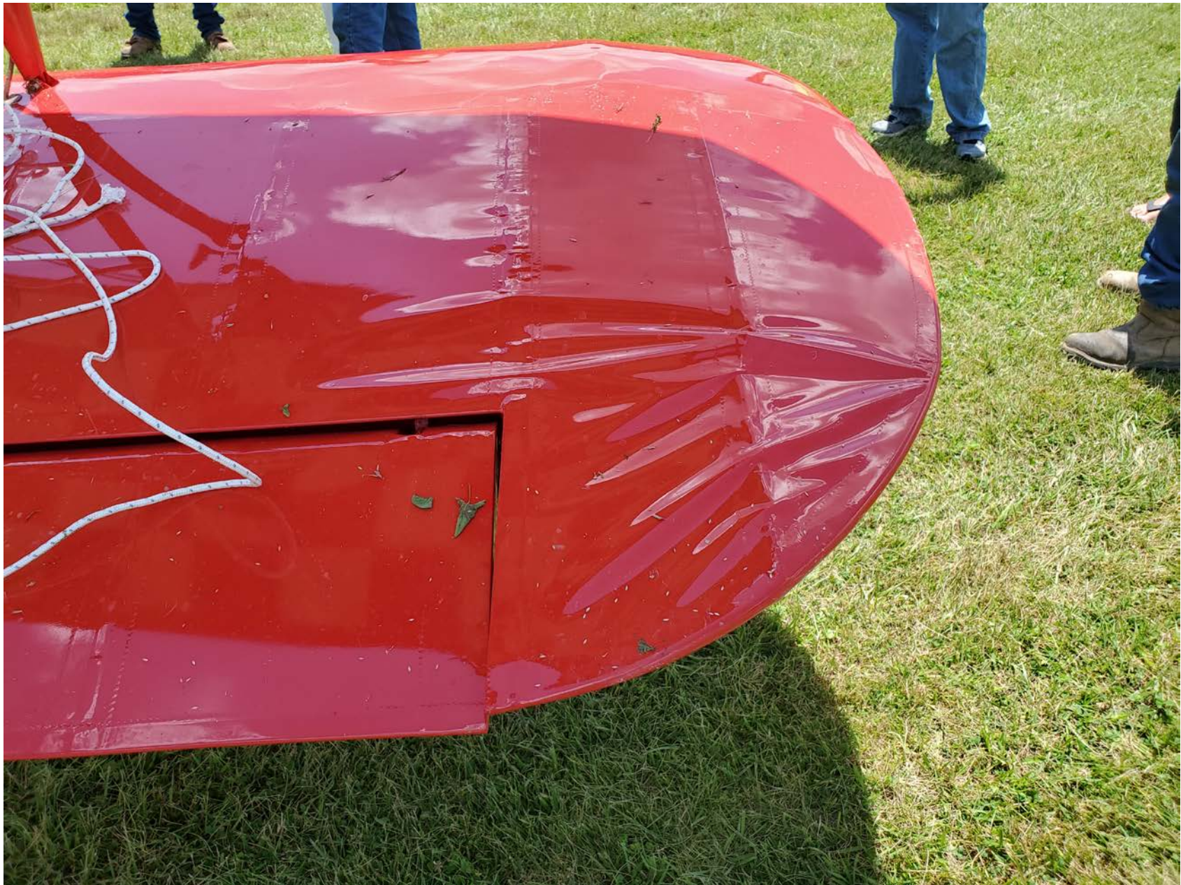
Photo 2 – Damage to right lower wing (Photo provided by FAA)
