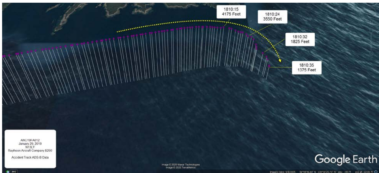
Figure 4 - A graphic showing the accident sequence.
