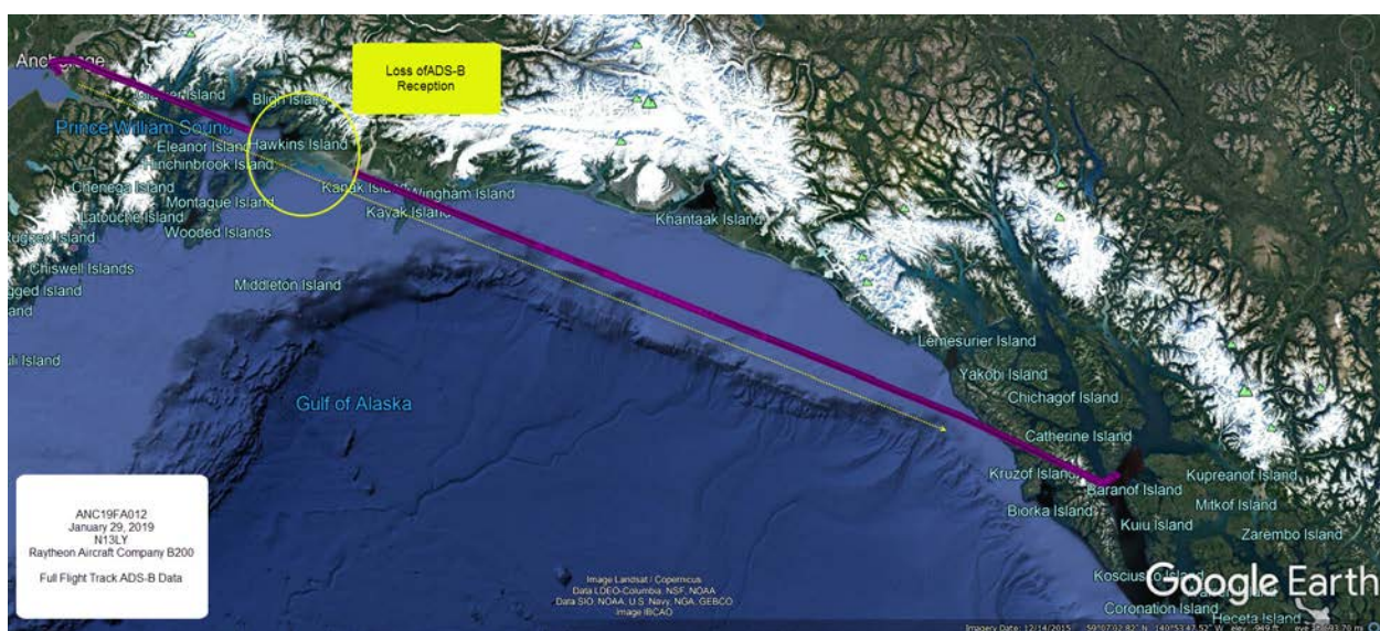
Figure 2 - A graphic showing the ADS-B flight of the entire flight.
