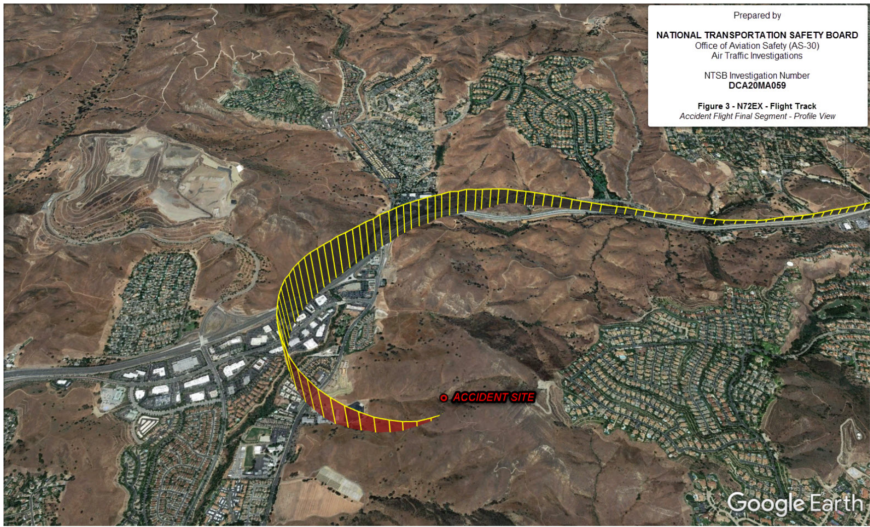
Figure 3 - Final segment of N72EX flight track in profile view illustrating the helicopters final climb and descending turn into terrain.
