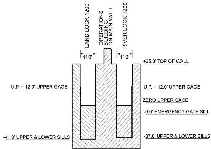
McAlpine Locks ELEVATION LOOKING DOWNSTREAM ELEVATION SHOWN IN FEET ABOVE ELEV. 408.0
