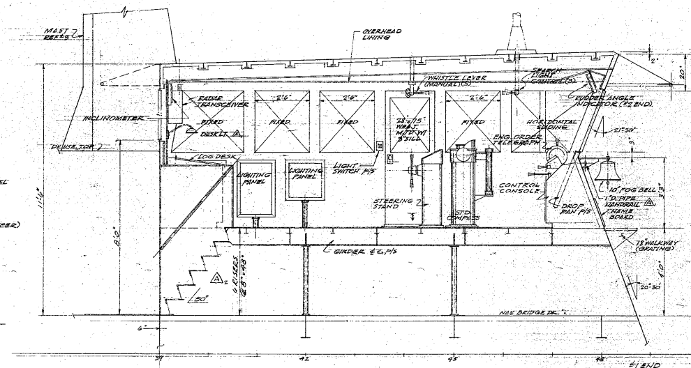
SECTION C-C (FR 19 LOCKING PORT)
