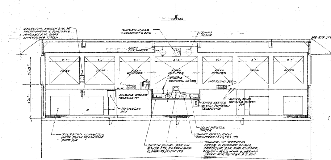
SECTION AA (FR 19 LKG FORWARD)
