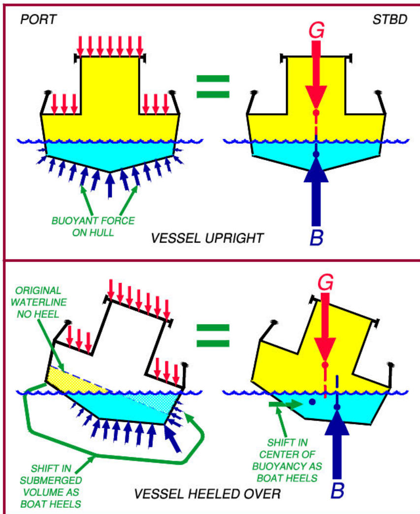
SHIFTING VOLUME AS THE VESSEL HEELS
