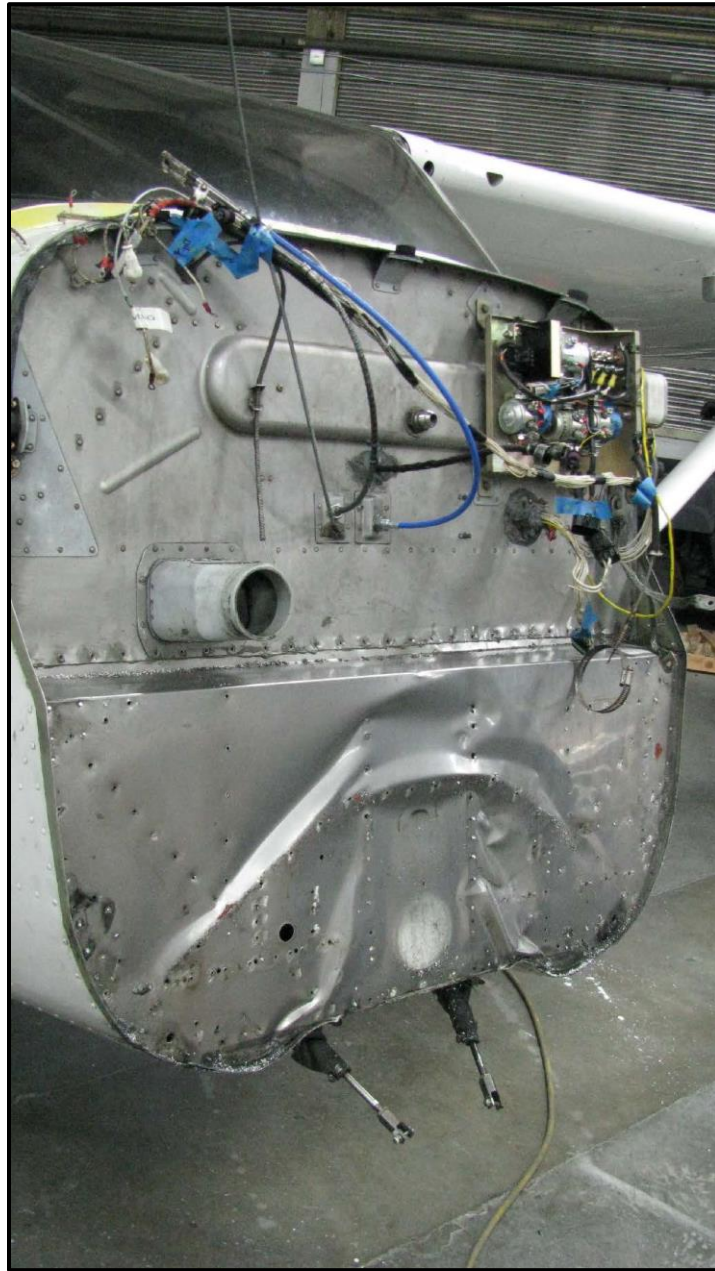
Photo 4 – Firewall (Elmendorf Aero Club Photo)
