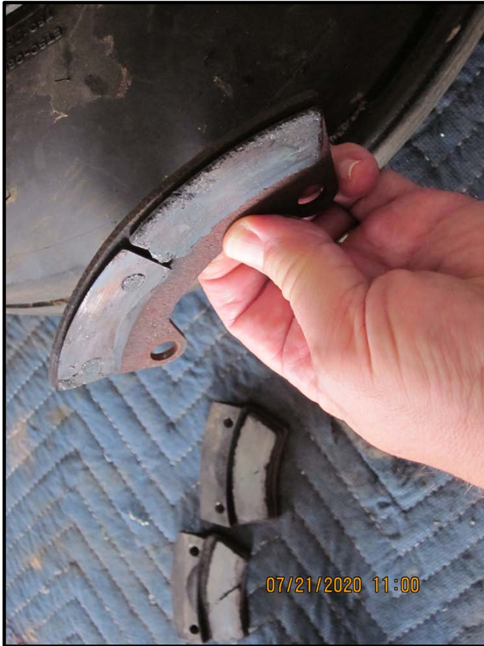
Photo 5 – Left Brake Pads (FAA Photos)
