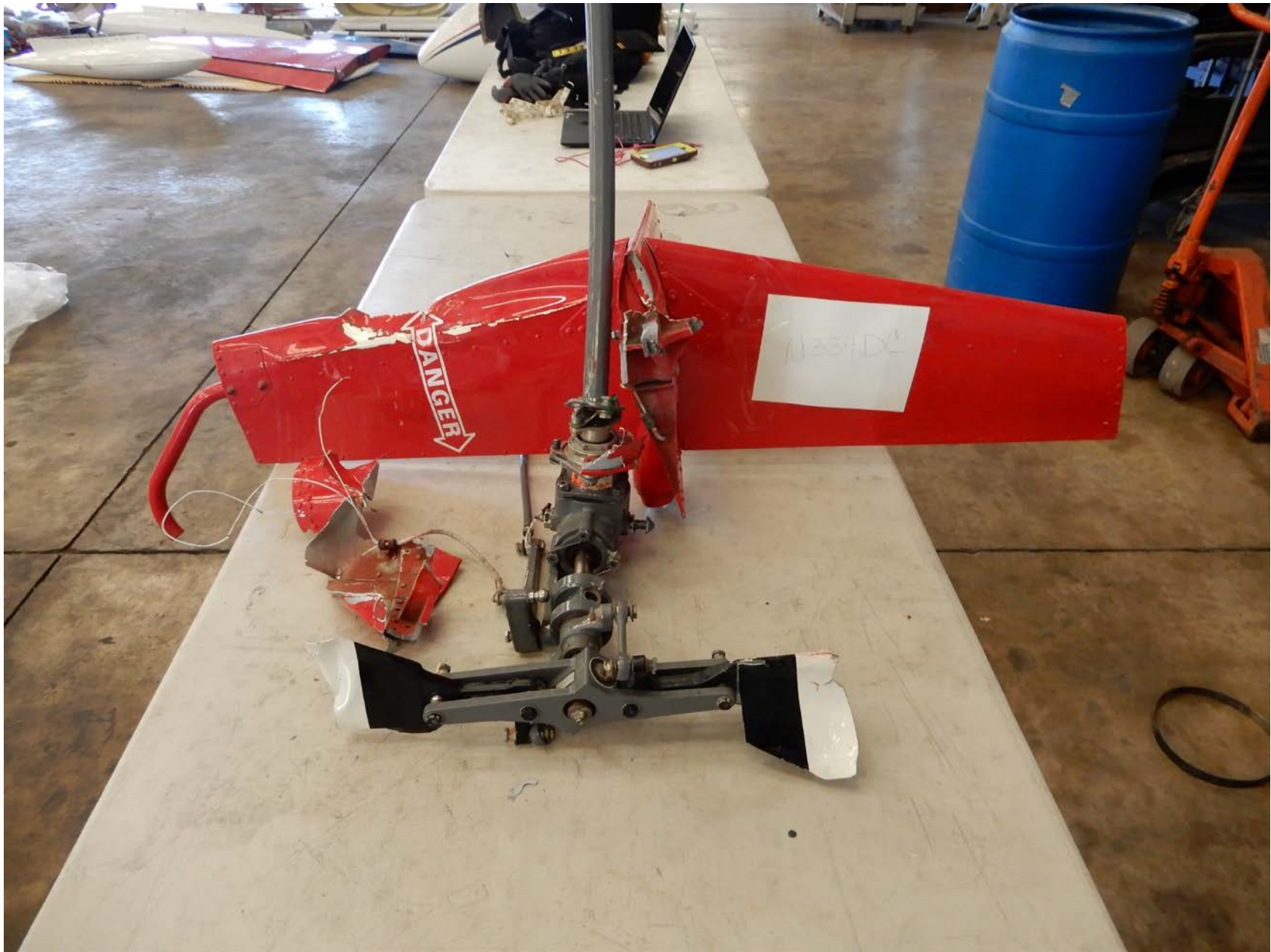
Photograph 2 – Vertical Fin and Tail Rotor Assembly
