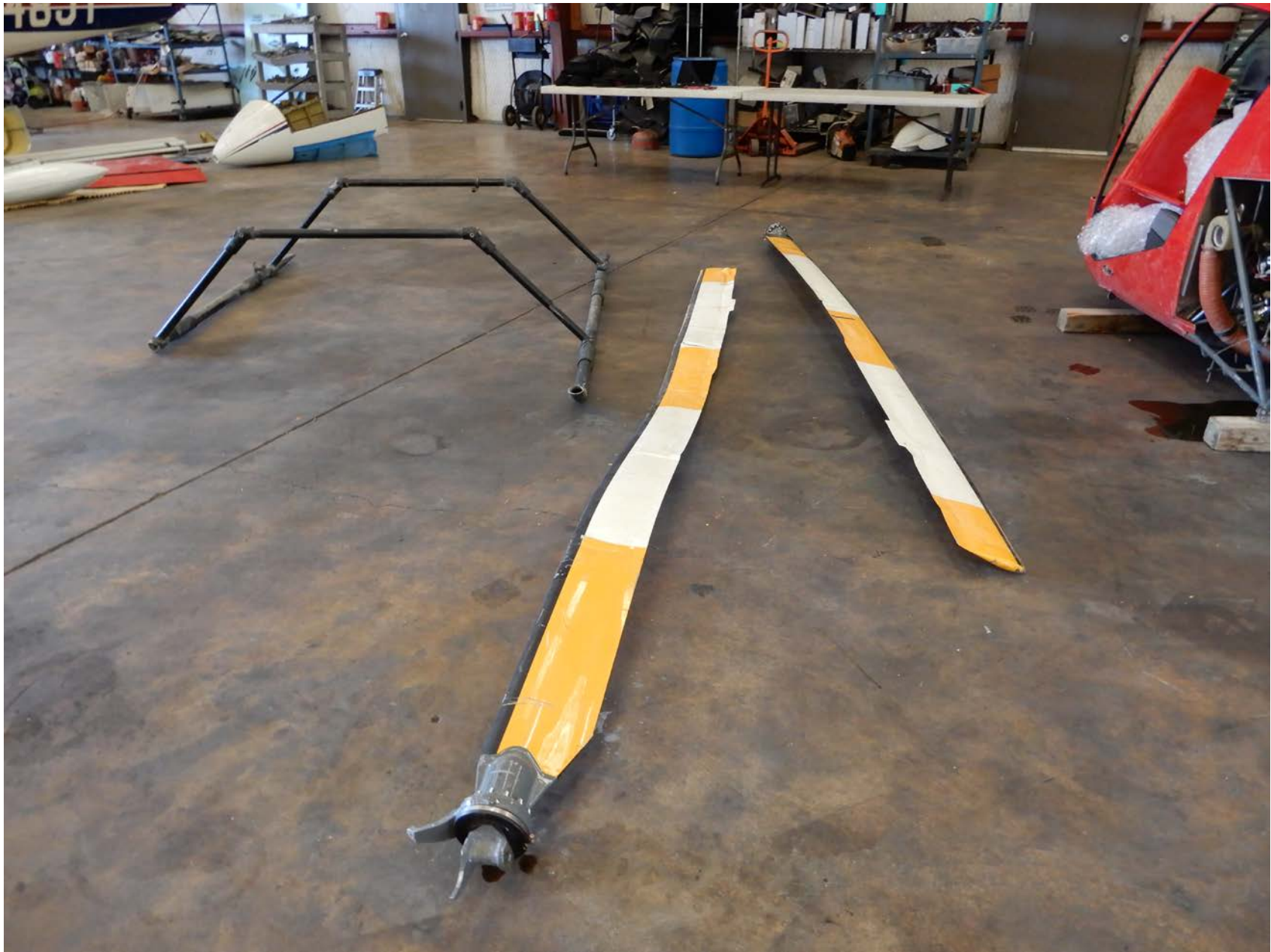
Photograph 3 – Main Rotor Blades
