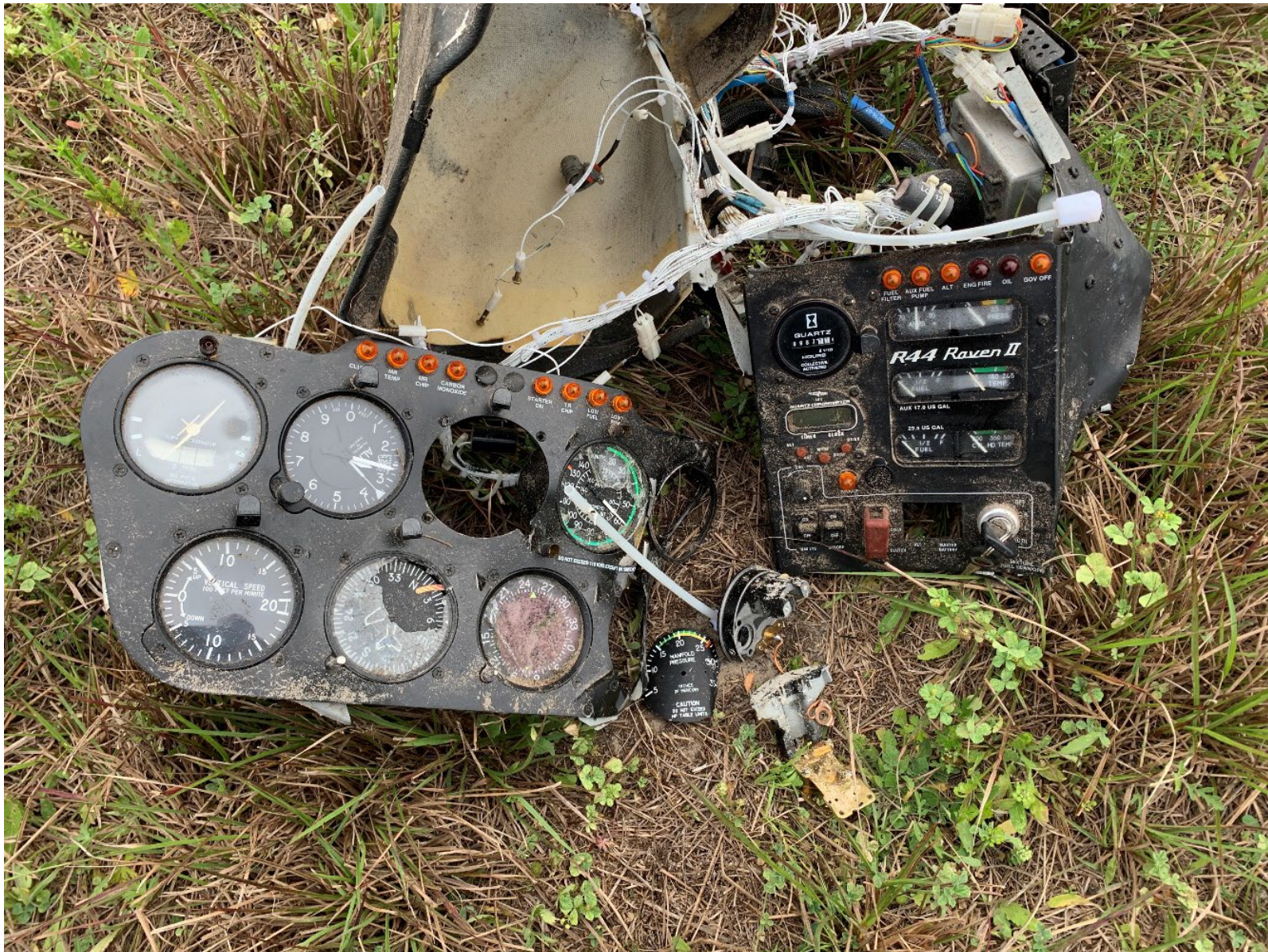
Photograph 8 - View of the instrument panel.
