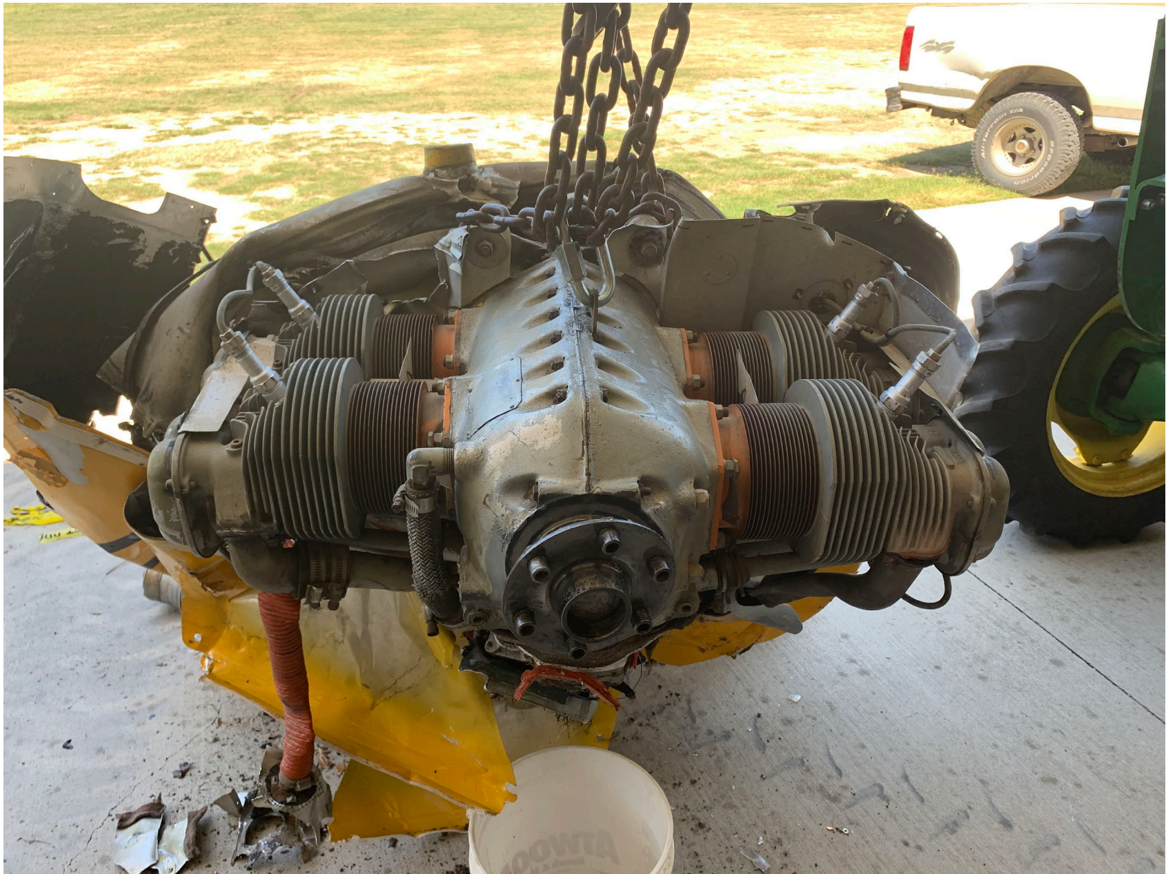
Photo 9 – View of the front of the engine during the examination.
