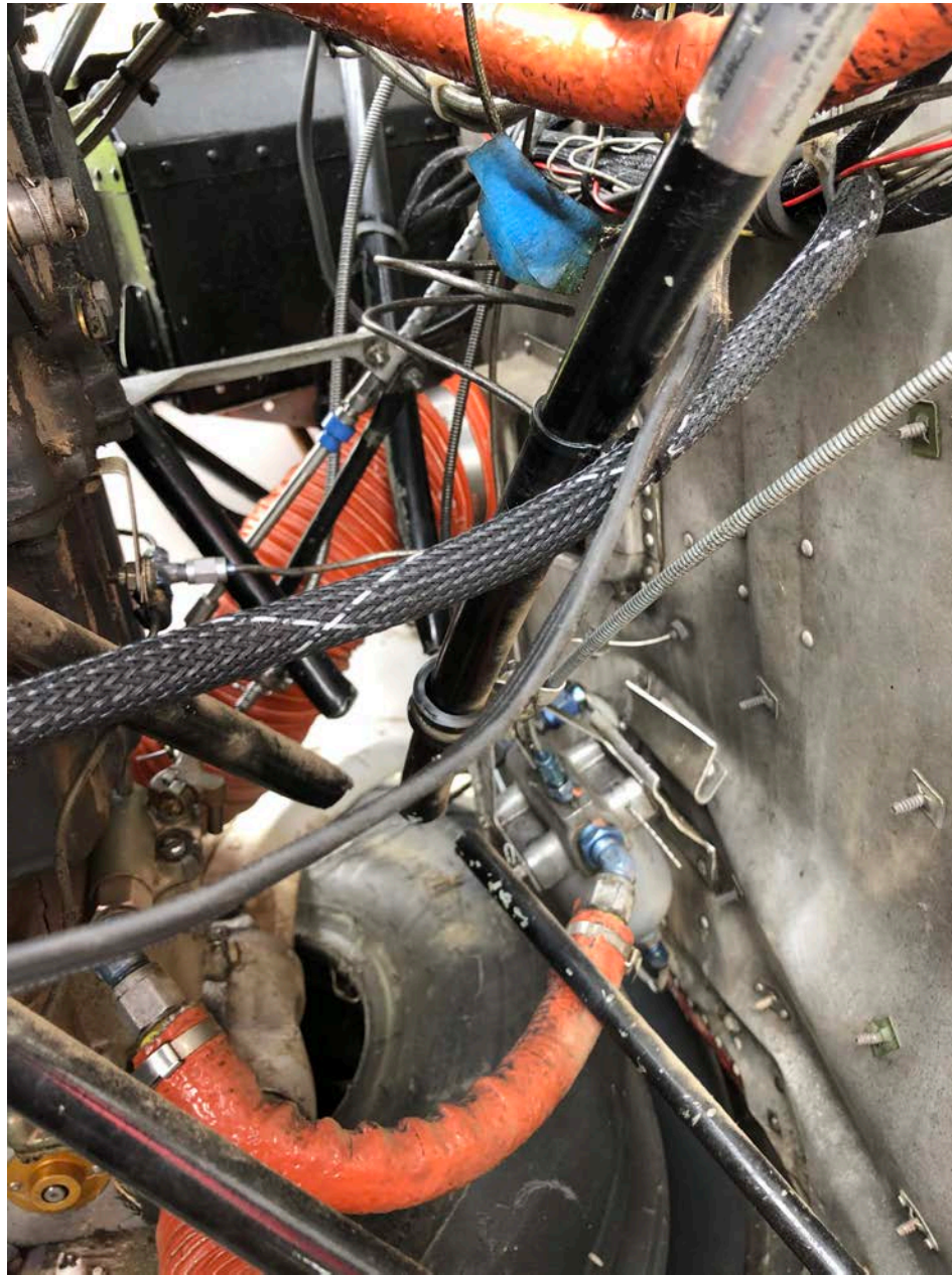
Photo 1 – View of damaged engine truss (courtesy of the FAA)
