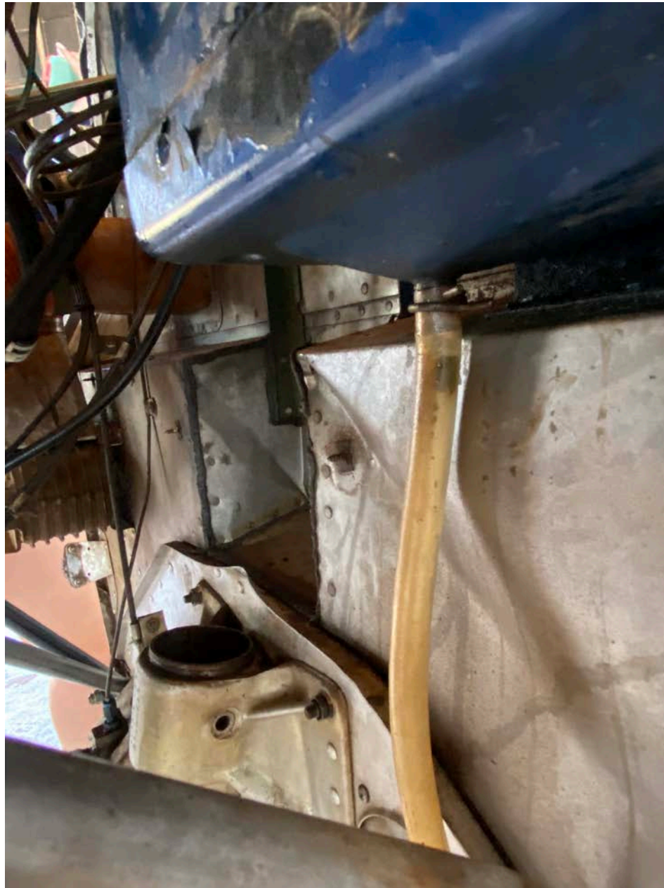
Photo 1 – View of damaged firewall and structure aft of the nose landing gear (courtesy of the FAA)
