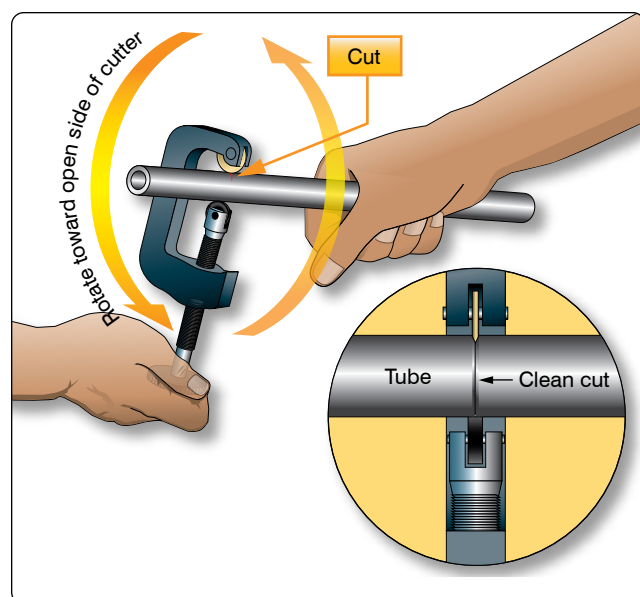
Figure 9-2. Tube cutting.
