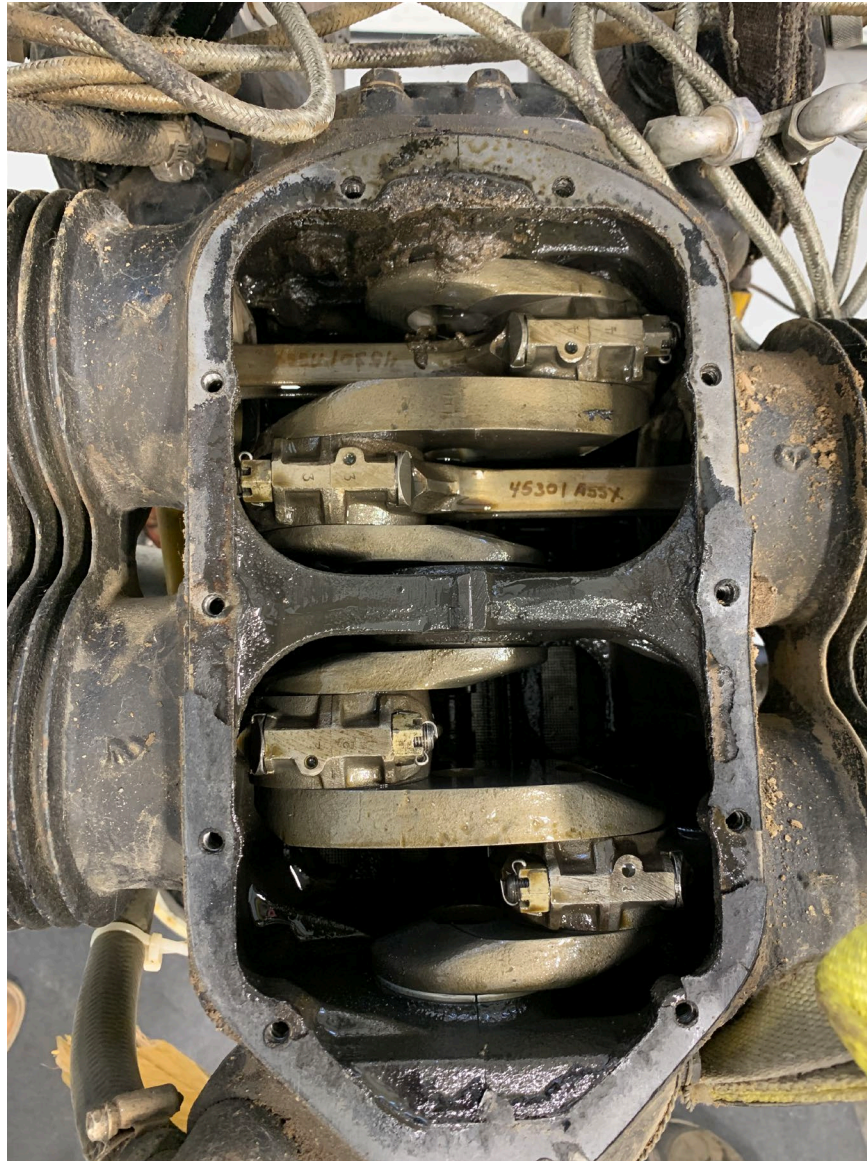
Photograph 5 - Top view of engine with top case removed during engine examination
