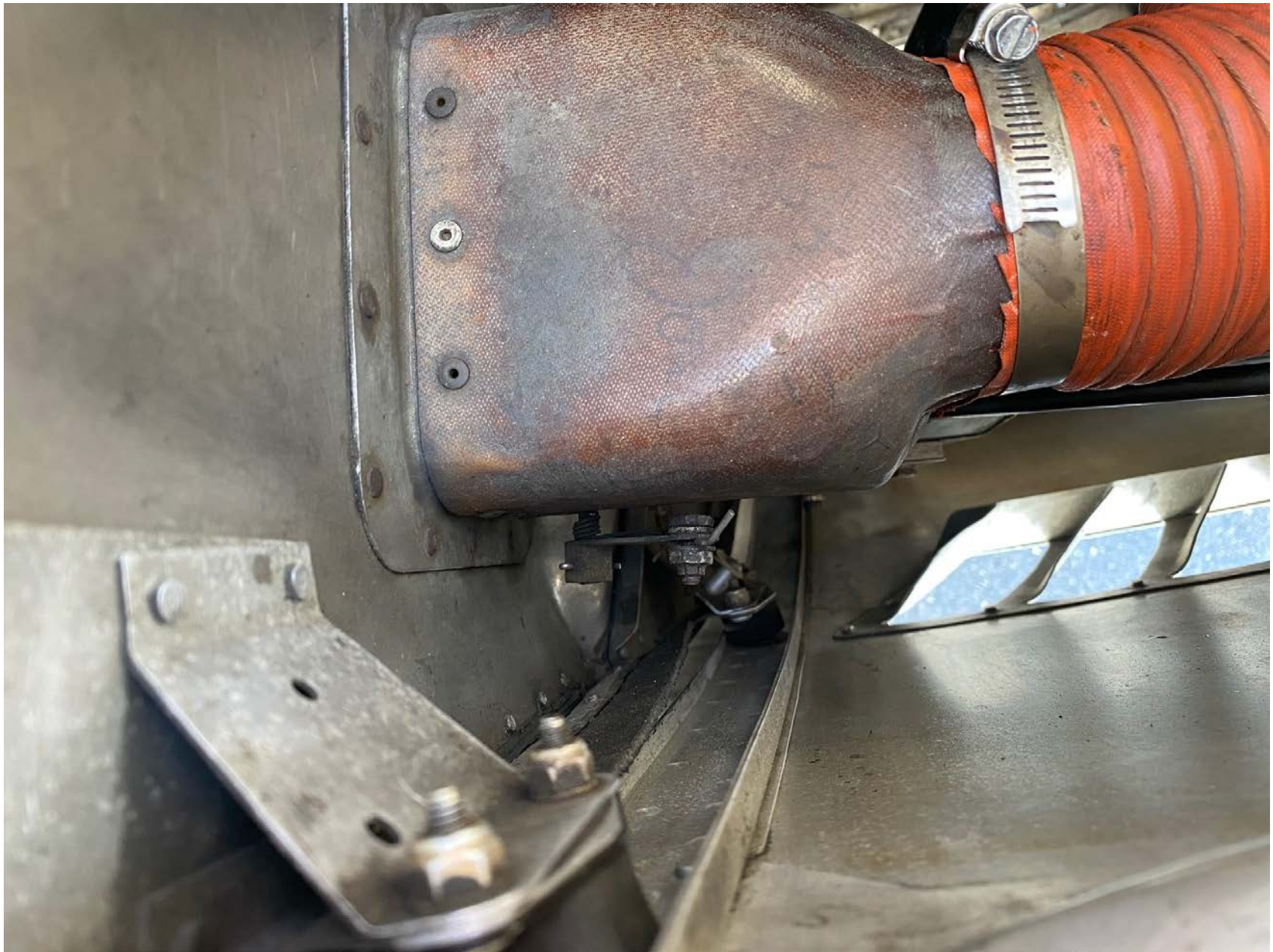
Photo 2 – Engine Firewall (FAA Photo)
